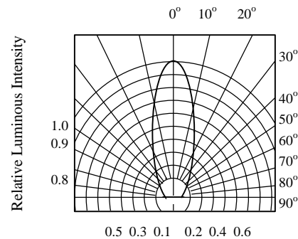
FIG.6 RADIATION DIAGRAM
