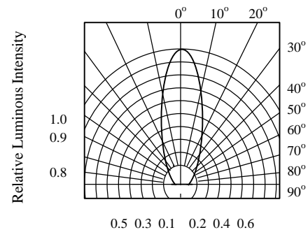
FIG.6 RADIATION DIAGRAM
