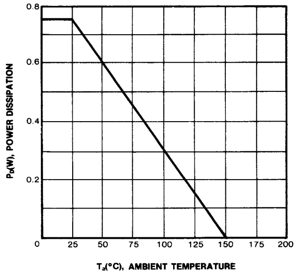
POWER DERATING
