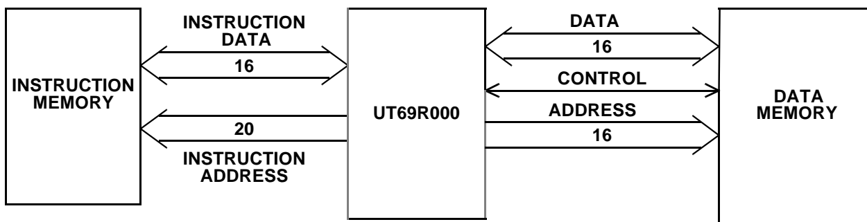
Figure 3. UT69R000 General System Architecture
