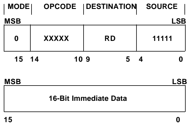
Figure 31c. Register Immediate Instruction Format
