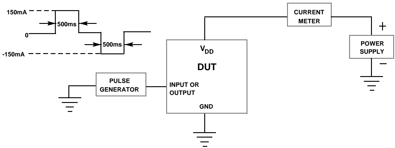
Figure 42. Latchup Test
