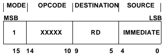
Figure 31b. Register to-Short Immediate Instruction Format
