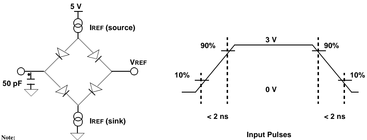
Figure 32b. AC Test Loads and Input Waveforms
