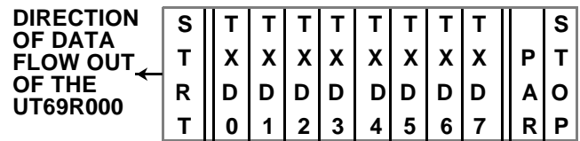
Figure 9. UART Transmitter Data String
