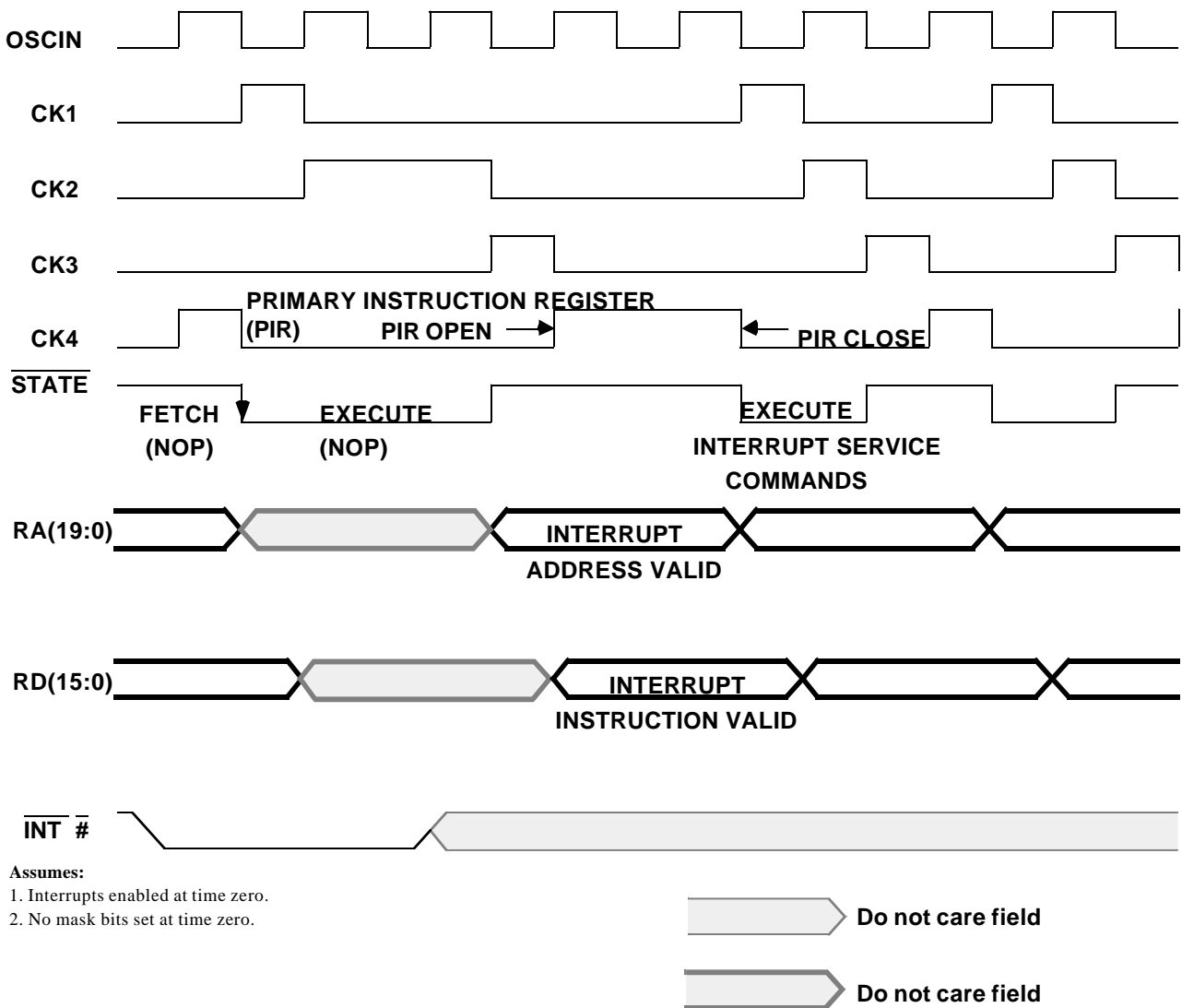
Figure 24. Interrupt Timing
