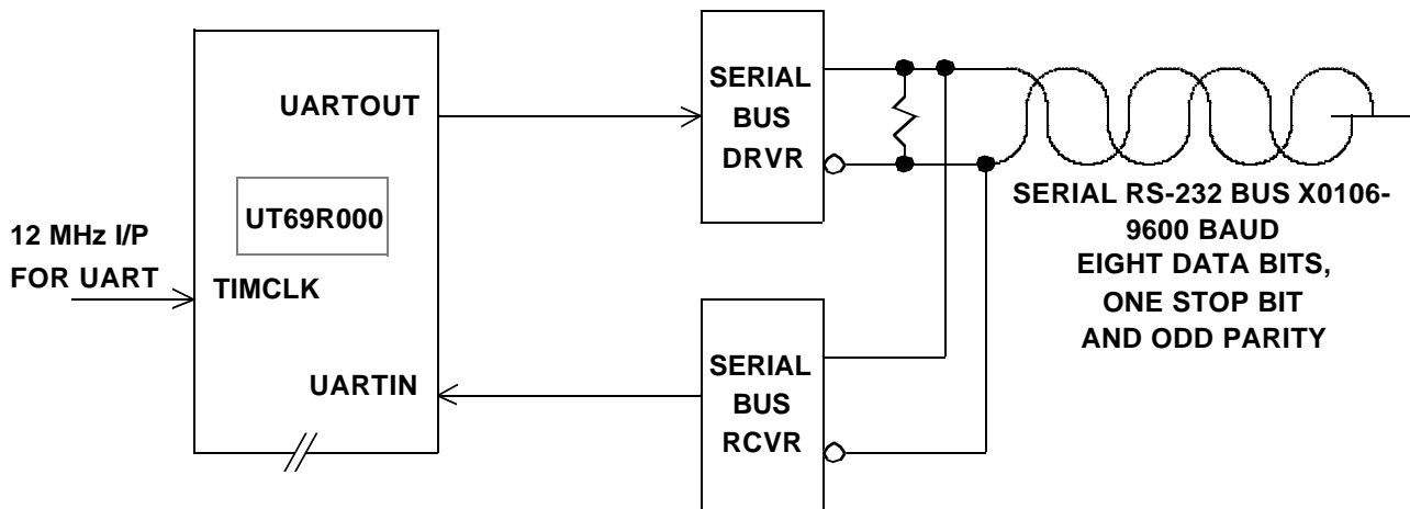
Figure 29. Serial Data Bus Interface to the UT69R000
