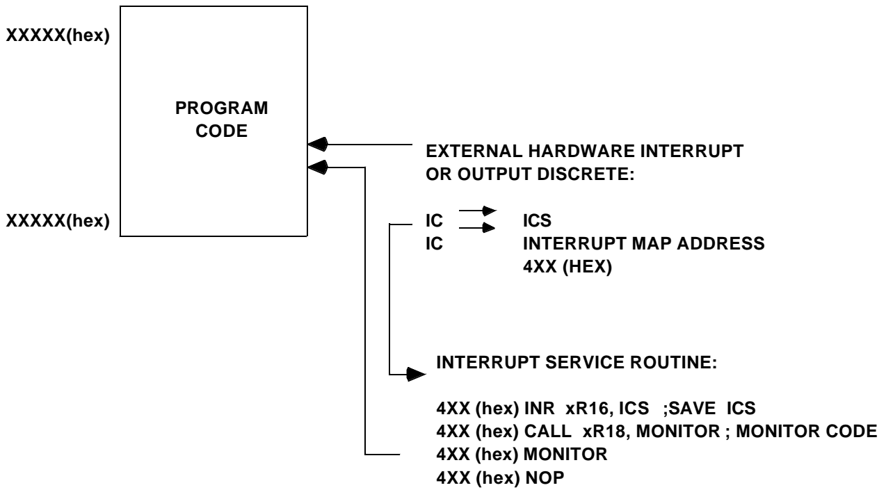
Figure 27. Monitor Operation
