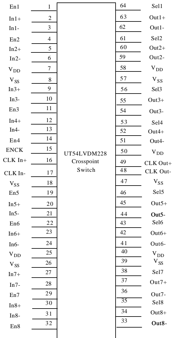
Figure 2. UT54LVDS228 Pinout
