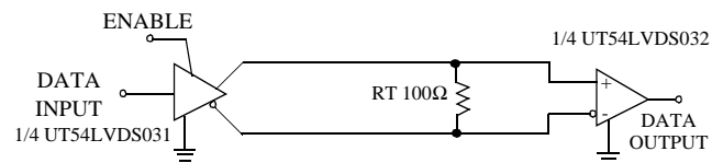
Figure 3. Point-to-Point Application
