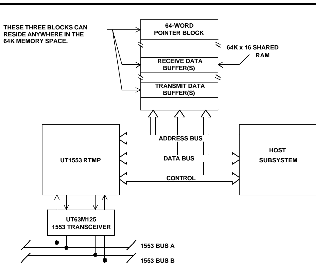
Figure 11. The Memory Link between the RTMP and the Host Subsystem
