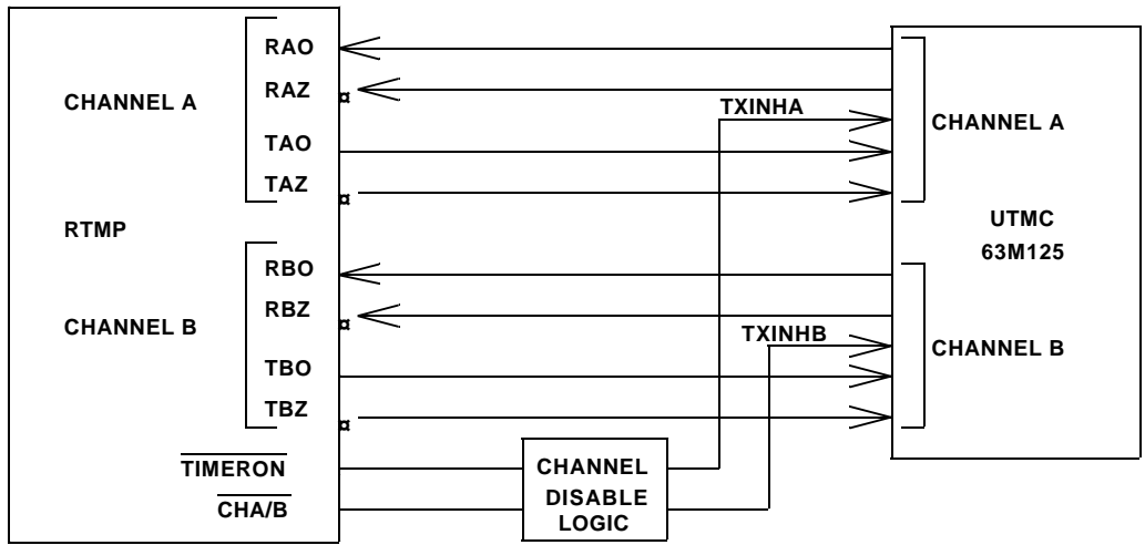
Figure 20. RTMP-to-Transceiver Interface Diagram
