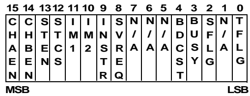
Figure 7. The Control Register in 1553B Mode
