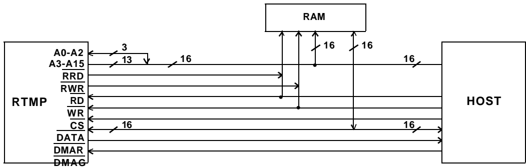
Figure 21. RTMP-to-Host Interface
