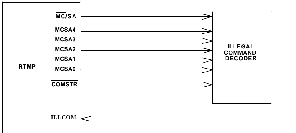
Figure 17. Mode Code/Subaddress Illegalization Circuit
