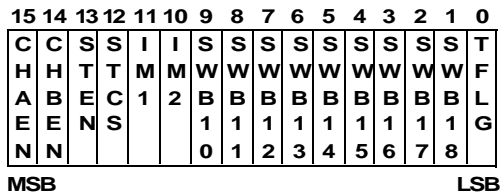
Figure 6. The Control Register in 1553A Mode
