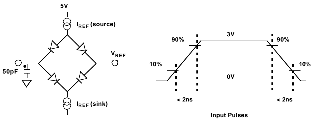
Figure 22. Typical Timing Measurements
