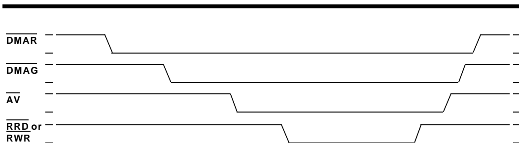
Figure 18. General RTMP DMA Timing Relationships
