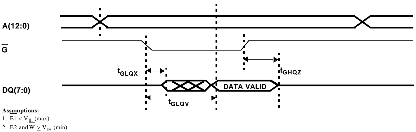
Figure 3c. SRAM Read Cycle 3: Output Enable Access
