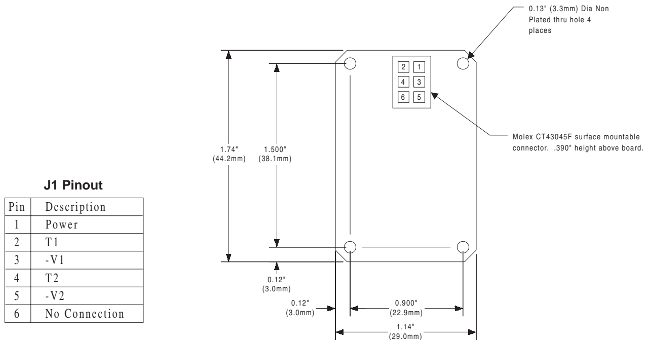
Figure 2. Mechanical Drawing
