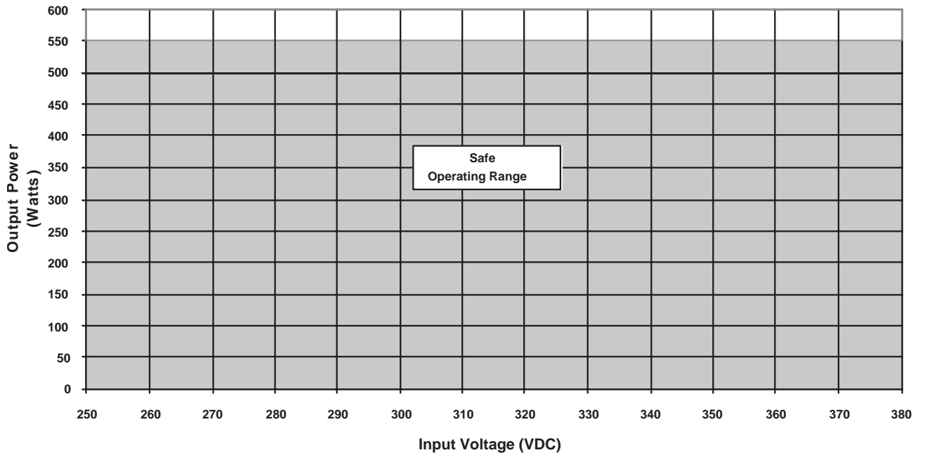
FlatPAC-EN Output Power vs. DC Input Voltage
