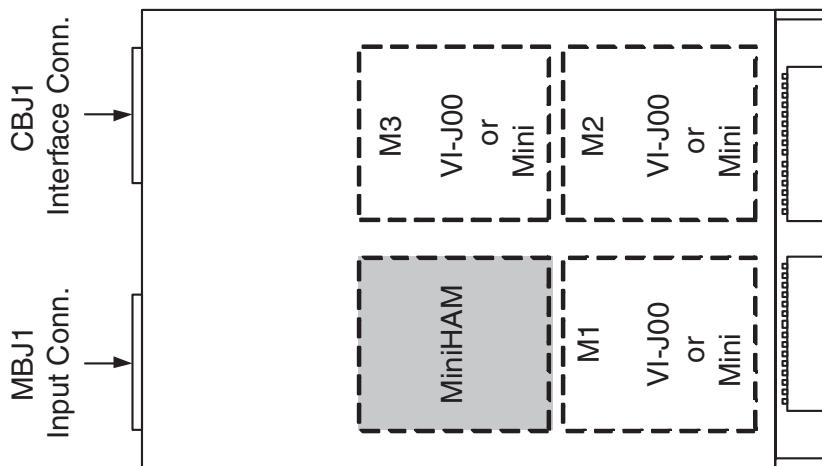
Triple Outputs (Two 18 pin Molex Connectors)
