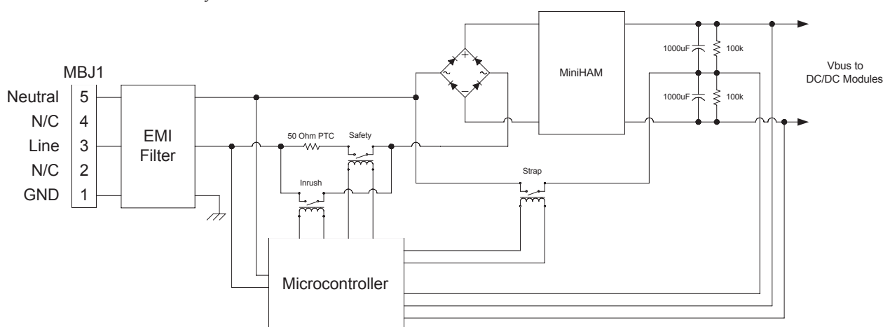
Figure 1. FlatPAC-EN Architecture
