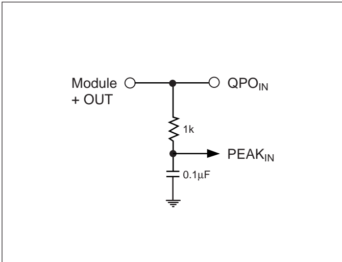
Figure 8 – Peak detector Disable Circuit
