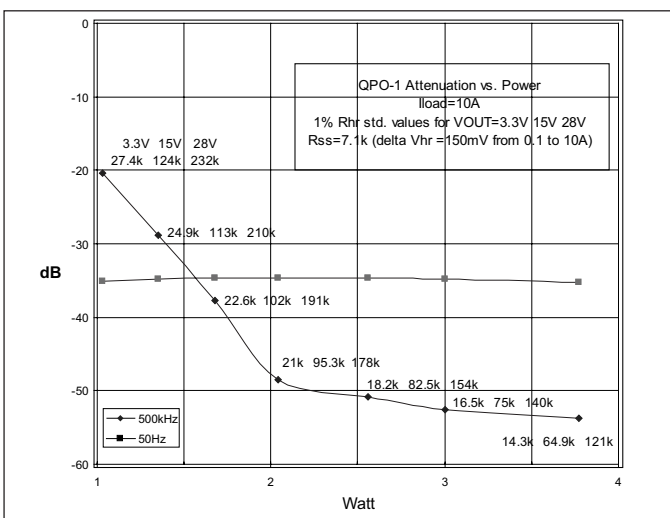
Figure 10 – Power vs Attenuation with slope adjust
