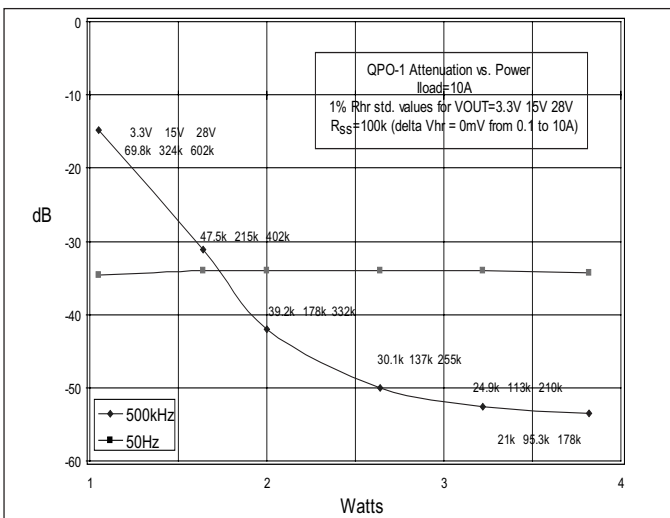
Figure 9 – Power vs Attenuation without slope
