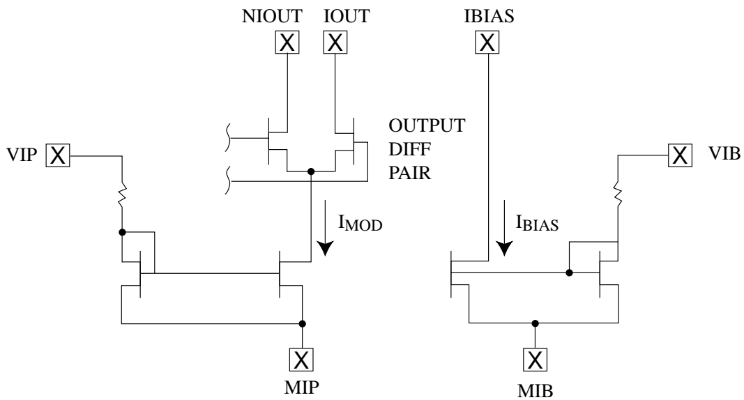
Figure 2: Simplified Output Structure
