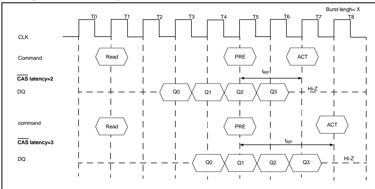
Precharge Termination in READ Cycle
