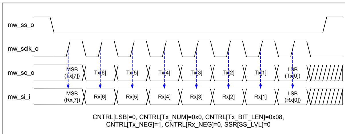
Fig. 6.19.1.1 USI Timing
