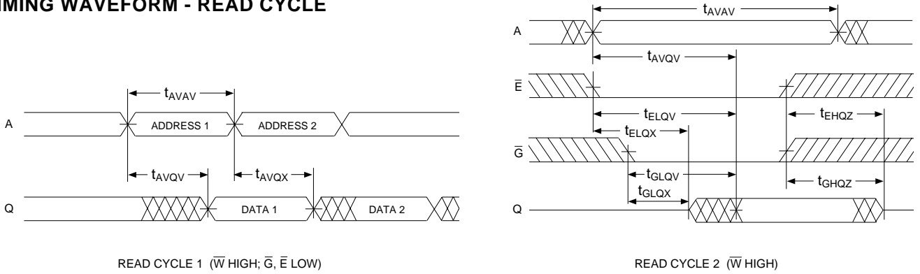
FIG. 2 TIMING WAVEFORM - READ CYCLE
