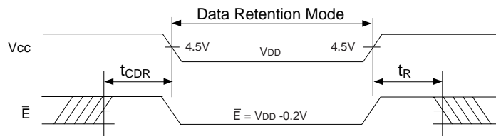
FIG. 5 DATA RETENTION - \bar{E} CONTROLLED
