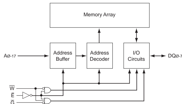
BLOCK DIAGRAM
