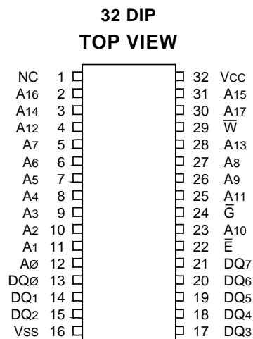
FIG. 1 PIN CONFIGURATION
