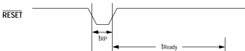
FIG. 3 RESET TIMING DIAGRAM
