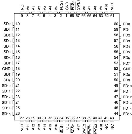
FIG. 2 PIN CONFIGURATION FOR WSF512K16-XG2X
