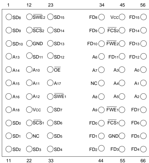
FIG. 1 PIN CONFIGURATION FOR WSF512K16-XH2X
