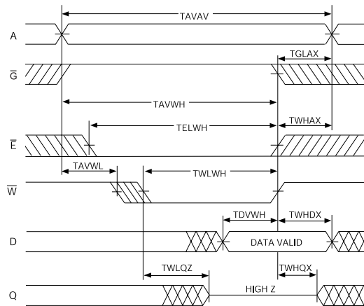
FIG. 6 WRITE CYCLE 1 - W CONTROLLED
