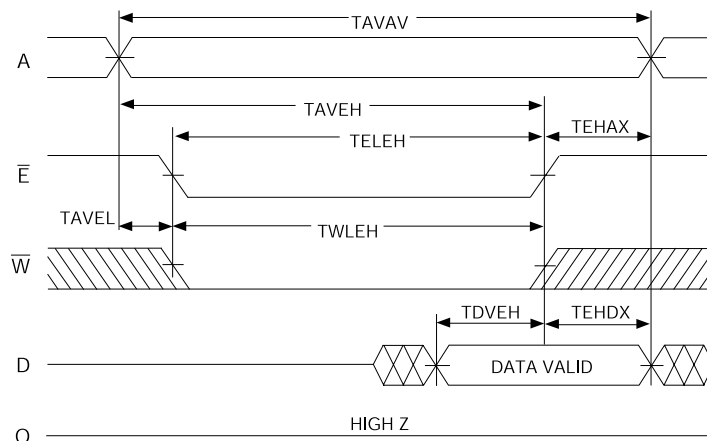
FIG. 7 WRITE CYCLE 2 - E CONTROLLED
