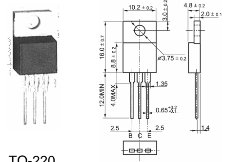
TO-220
