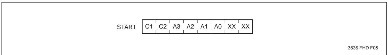
Figure 3. Control Byte
