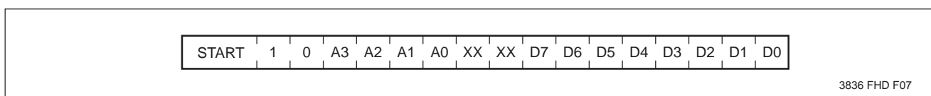
Figure 5. Read Sequence
