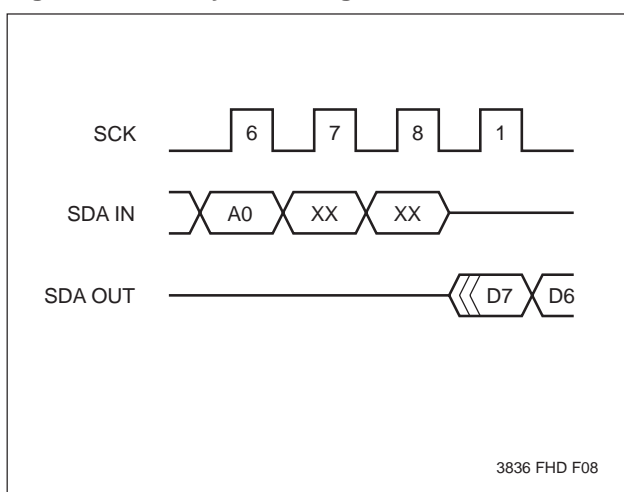
Figure 6. Read Cycle Timing
