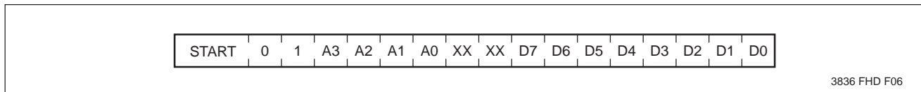
Figure 4. Write Sequence
