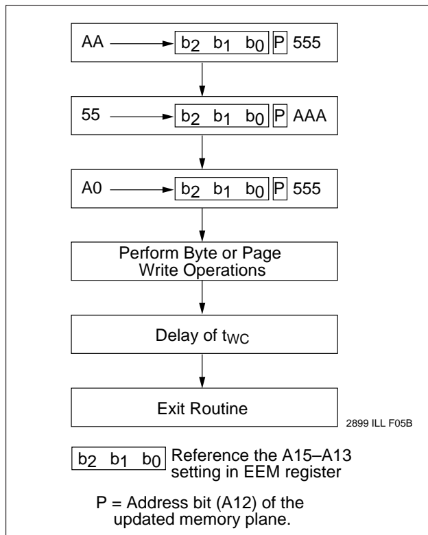
Figure 2. Writing with SDP Enabled
