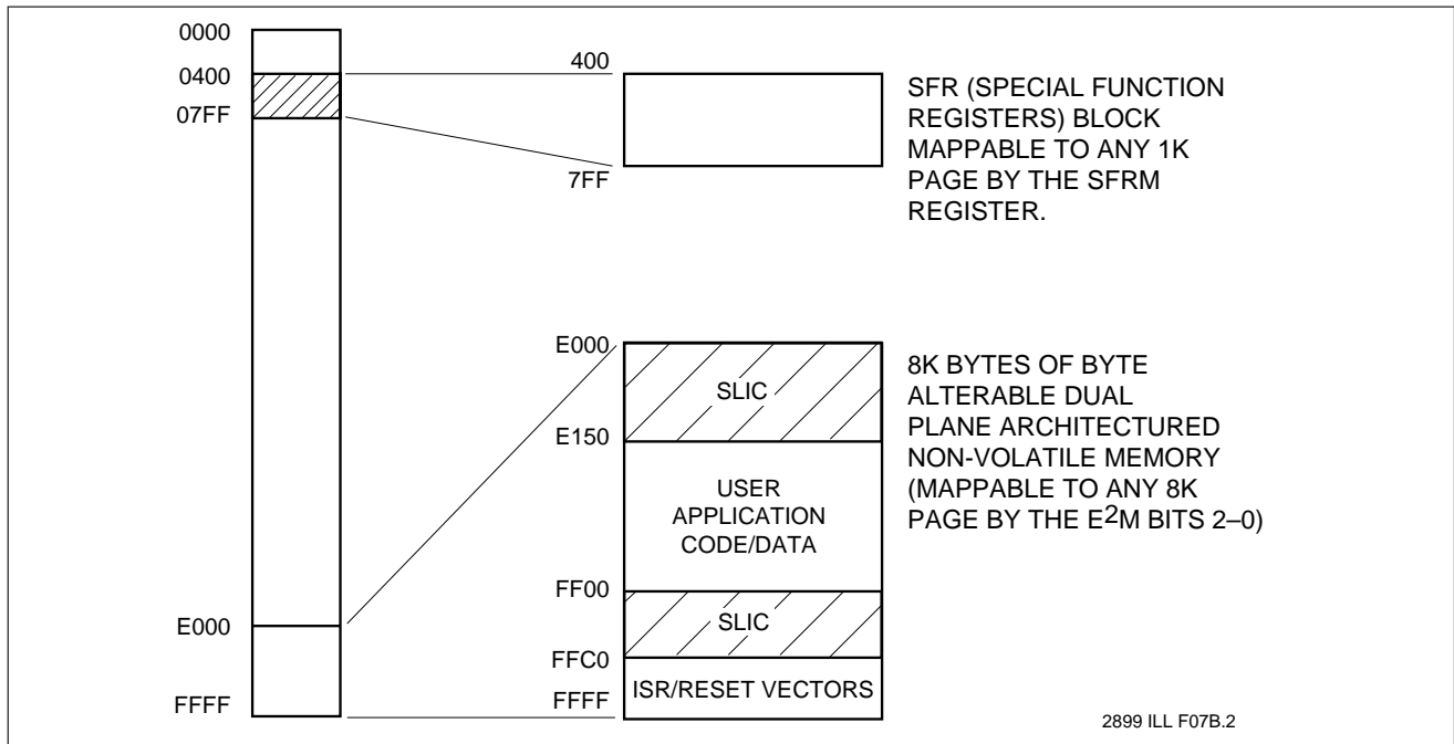
Figure 6. Microcontroller Map
