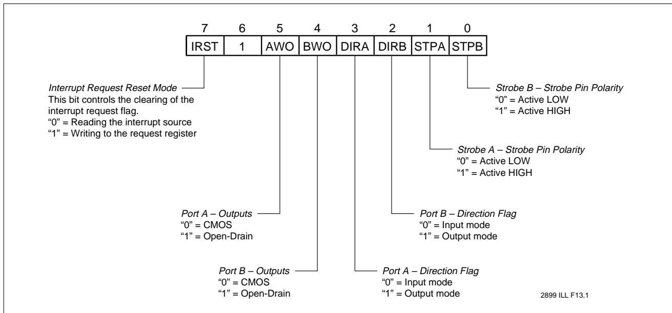
Figure 11. Configuration Register
