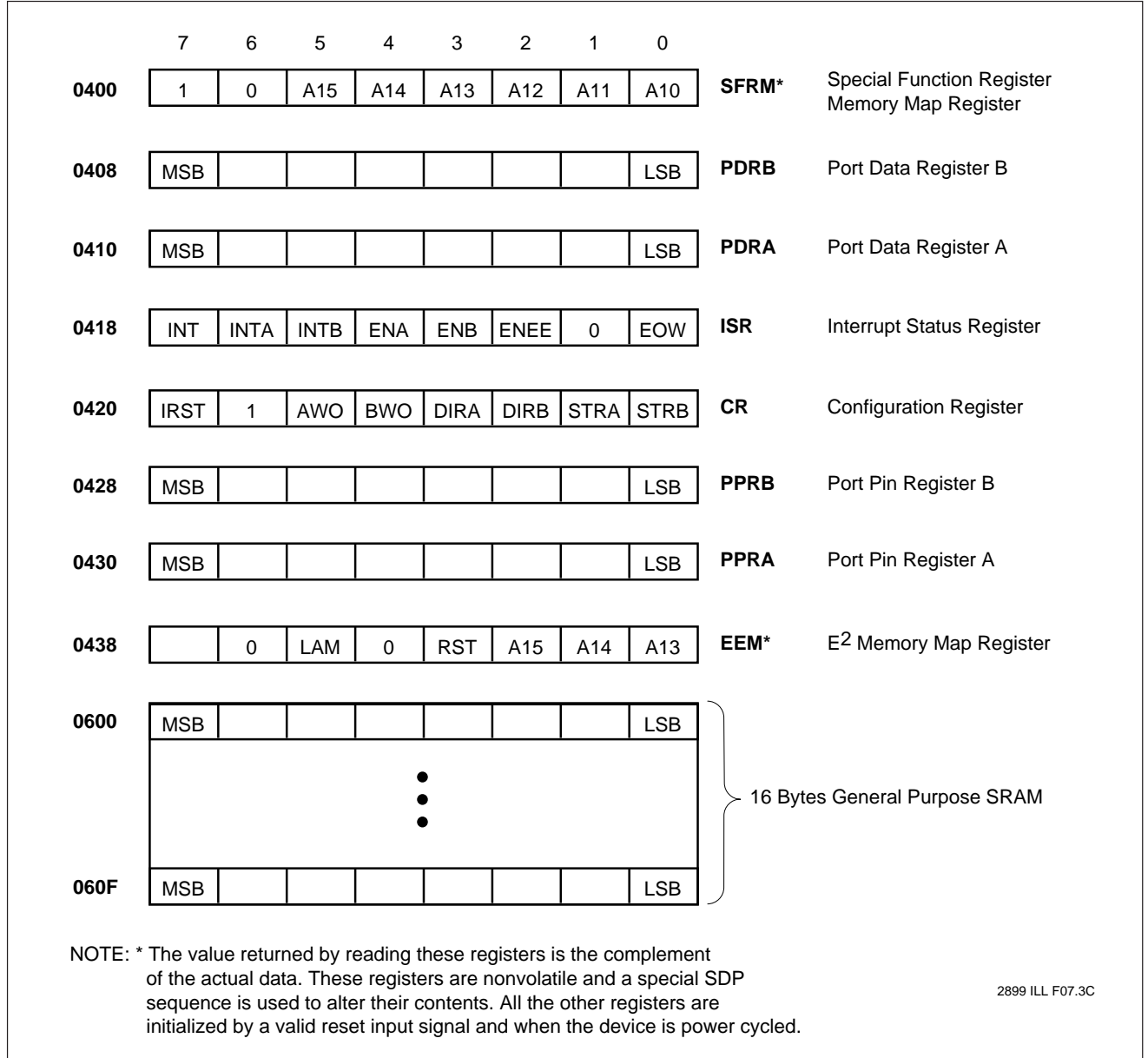
Figure 7. On-Chip Registers
