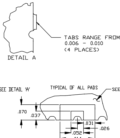
PHYSICAL DIMENSIONS
