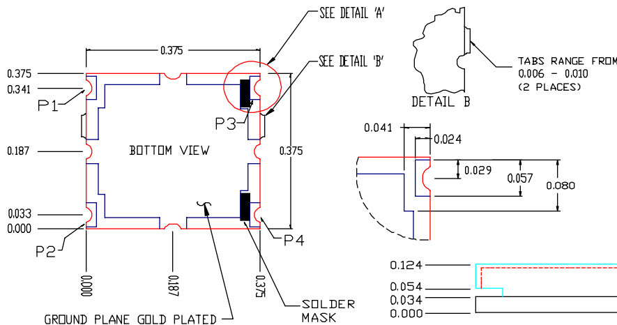
PHYSICAL DIMENSIONS
