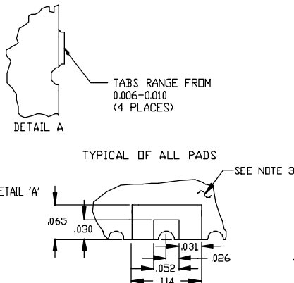
PHYSICAL DIMENSIONS
