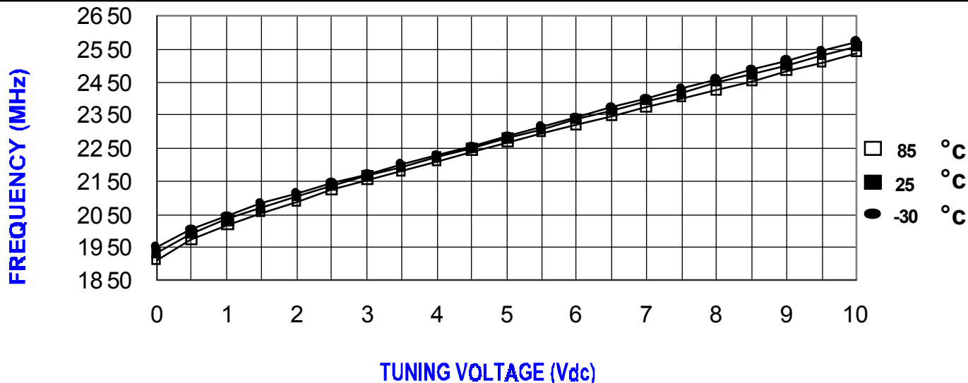
TUNING CURVE, typ.
