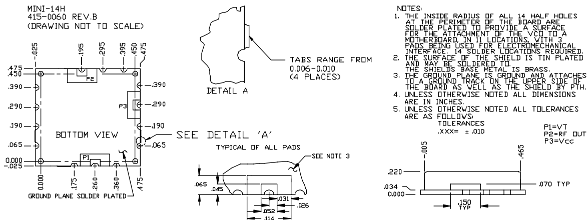
PHYSICAL DIMENSIONS
