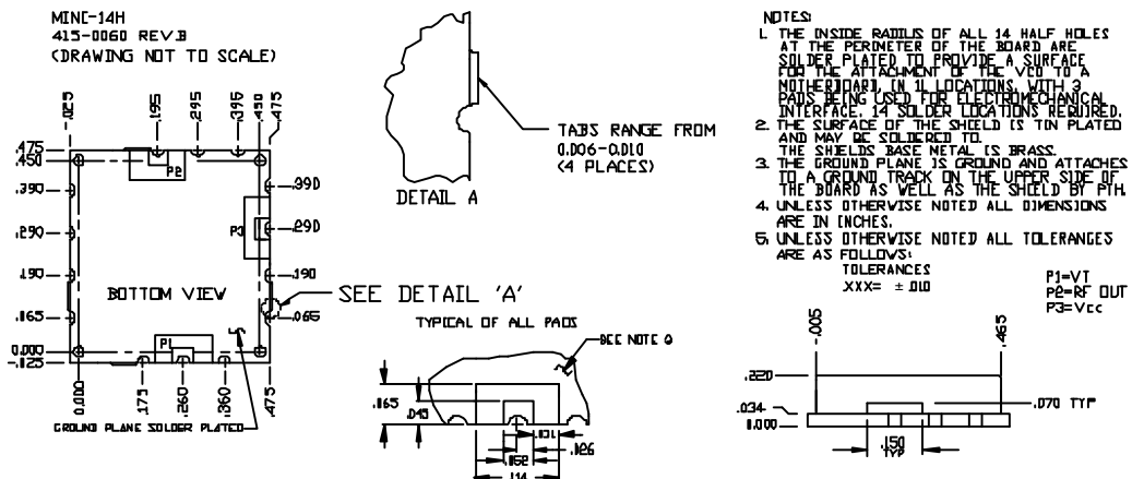
PHYSICAL DIMENSIONS
