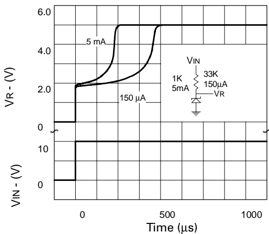
Transient Response (Single Pulse)
