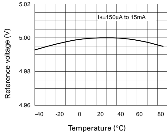
Temperature Drift
