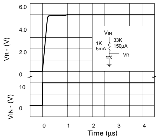
Transient Response (Repetitive Pulse)
