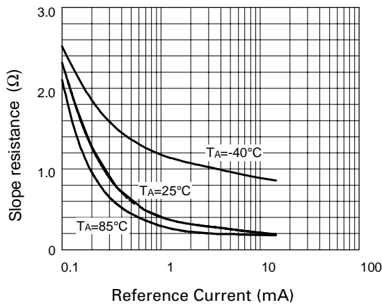
Slope Resistance v Current
