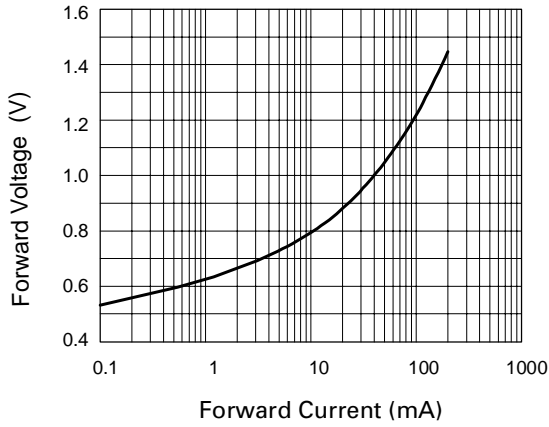
Forward Characteristics
