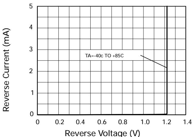
Reverse Characteristics
