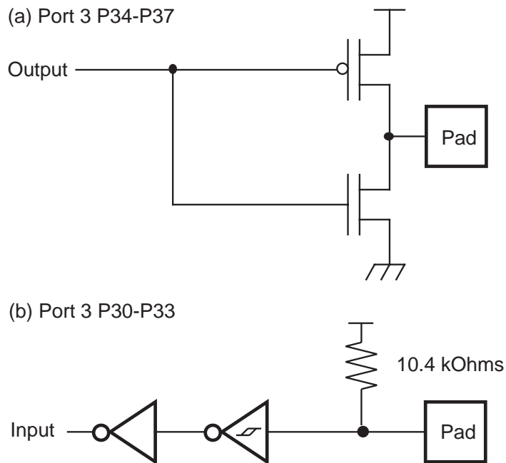
Figure 10. Port 3 Configuration
