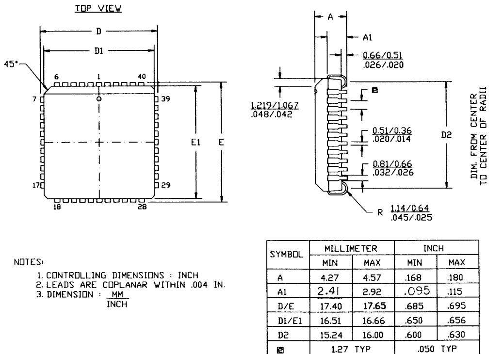
Figure 33. 44-Pin PLCC Package Diagram
