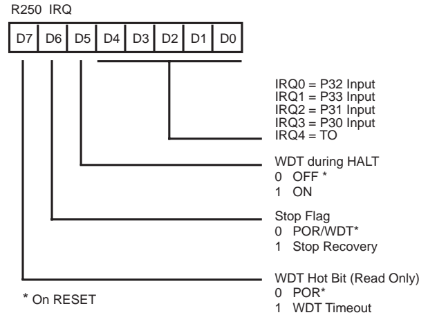
Figure 19. IRQ Register
