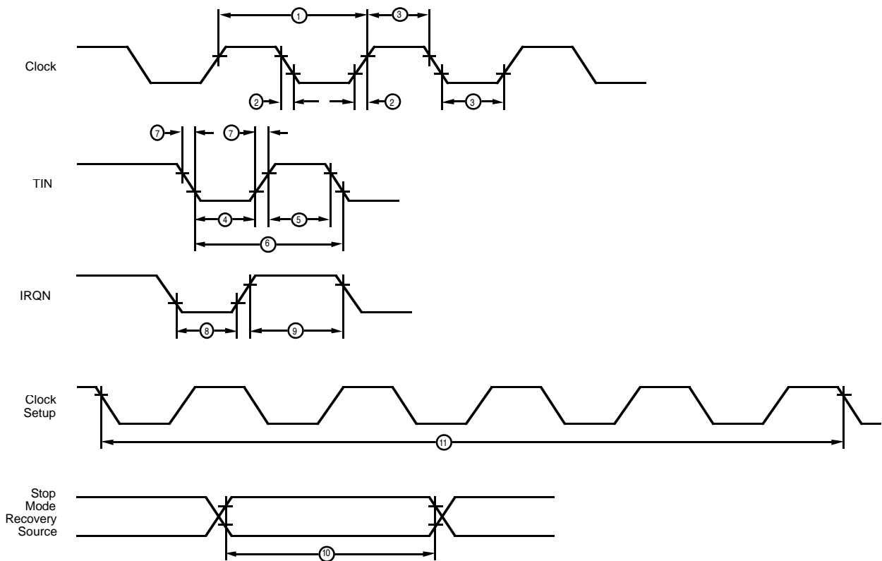
Figure 6. Additional Timing
