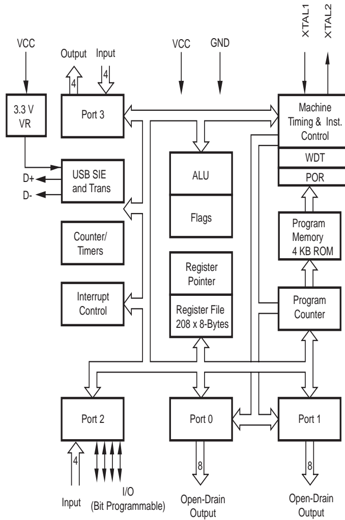
Figure 1. Z86KXX Functional Block Diagram
