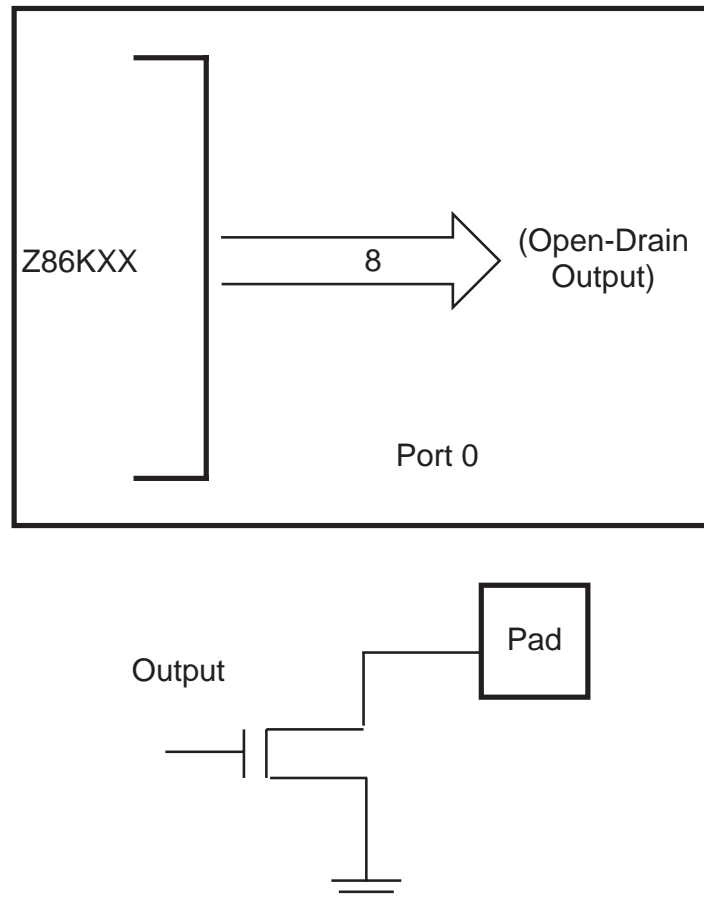
Figure 7. Port 0 Configuration
