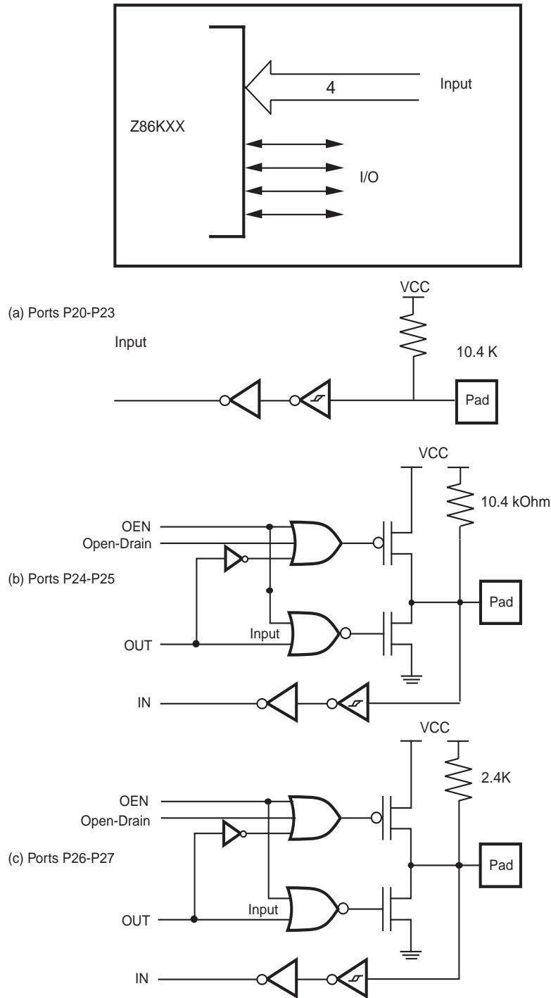
Figure 9. Port 2 Configuration
