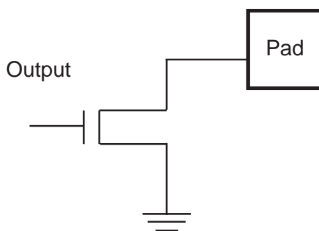
Figure 8. Port 1 Configuration
