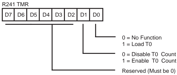
Figure 21. Timer Mode Register (F1 H : Read/Write)
