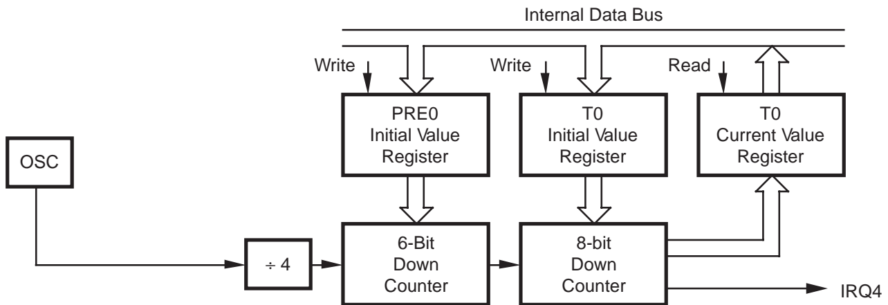
Figure 15. Counter/Timers Block Diagram
