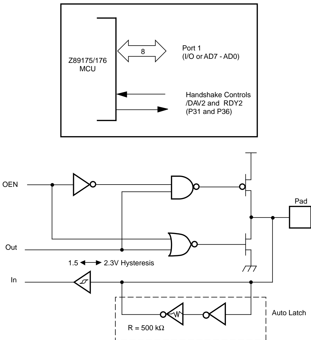
Figure 12. Port 1 Configuration
