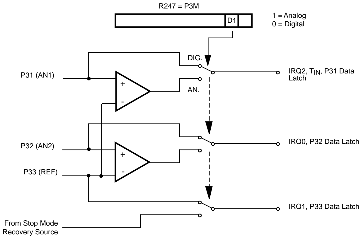
Figure 14. Port 3 Configuration
