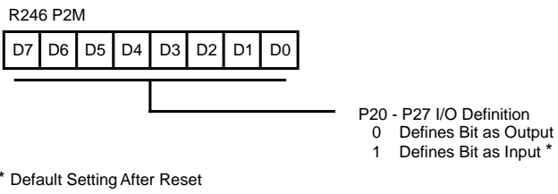
Figure 73. Port 2 Mode Register (F6H: Write-Only)
