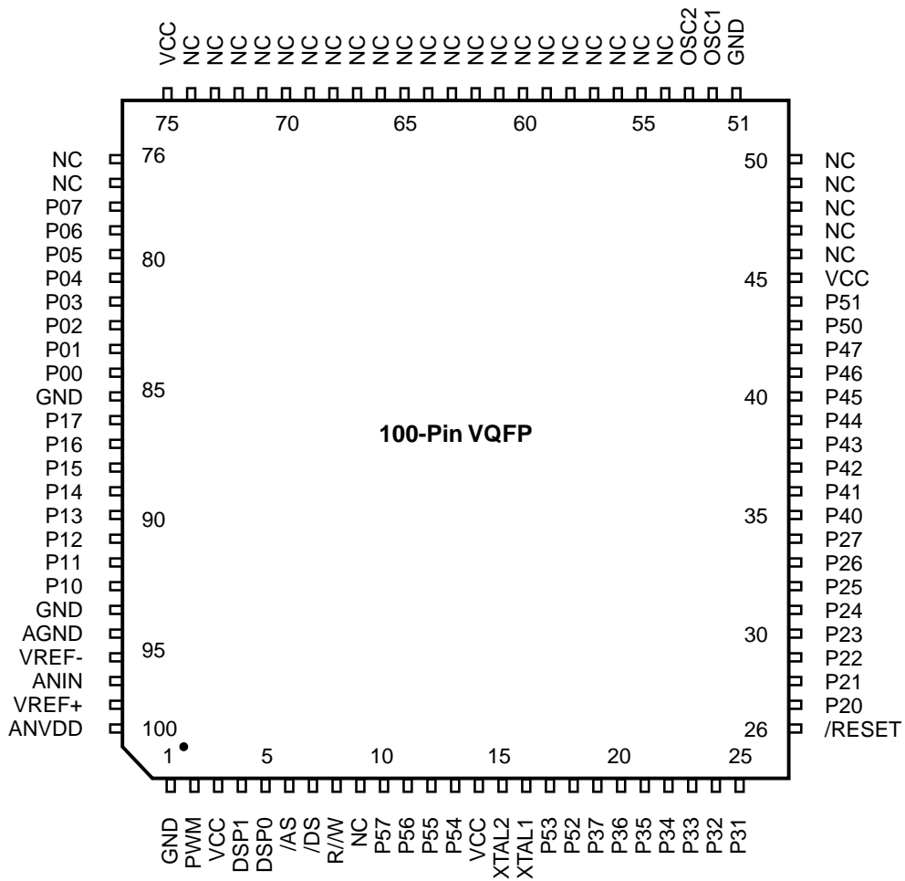
Figure 5. Z89176 100-Pin VQFP Pin Configuration
