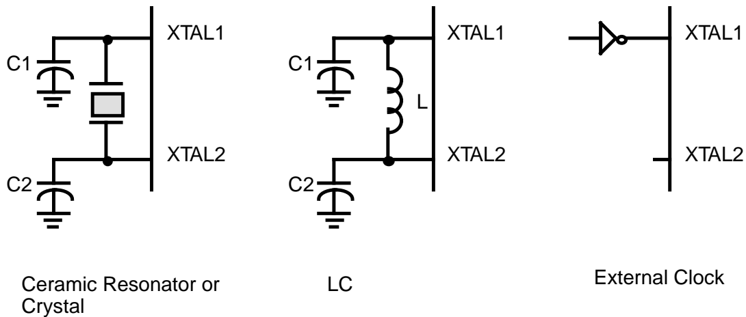
Figure 23. Oscillator Configuration
