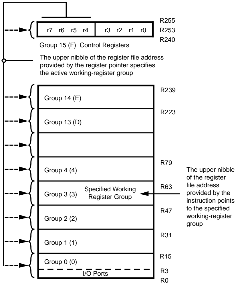
Figure 20. Register Pointer
