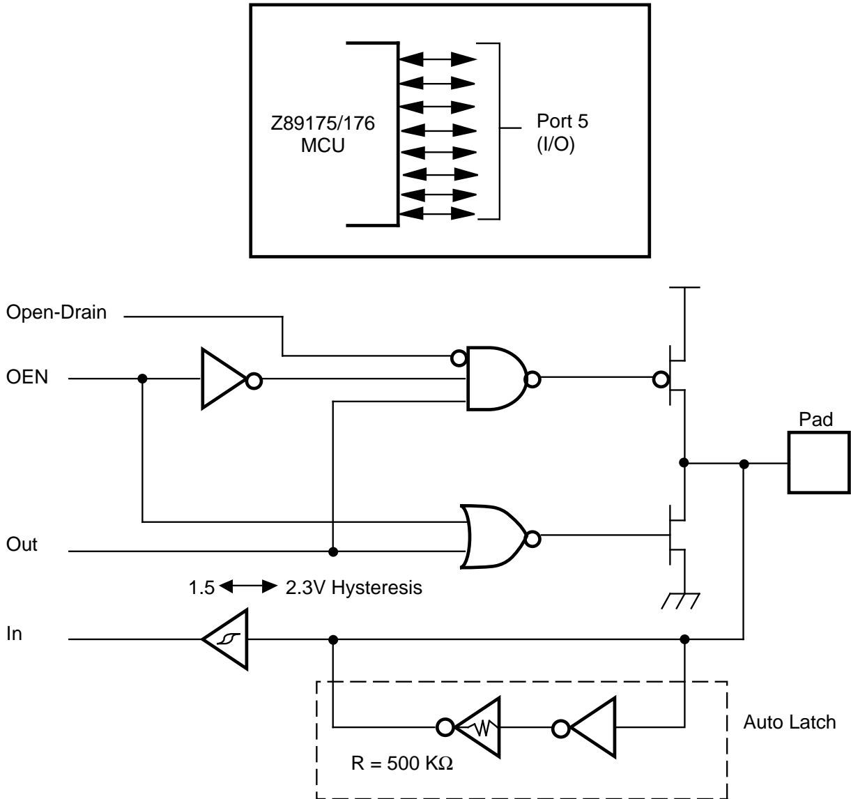
Figure 16. Port 5 Configuration
