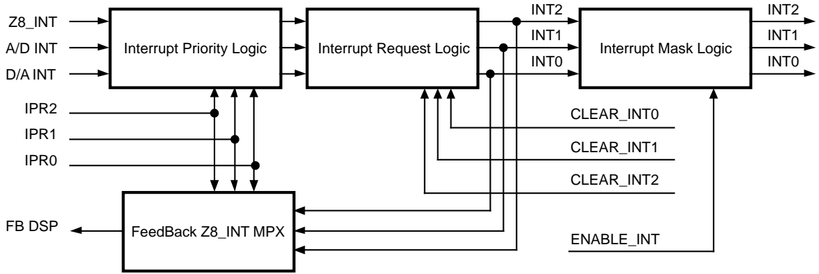
Figure 32. DSP Interrupts
