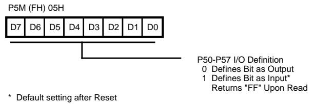
Figure 63. Port 5 Mode Register (F) 05H [Write-Only]
