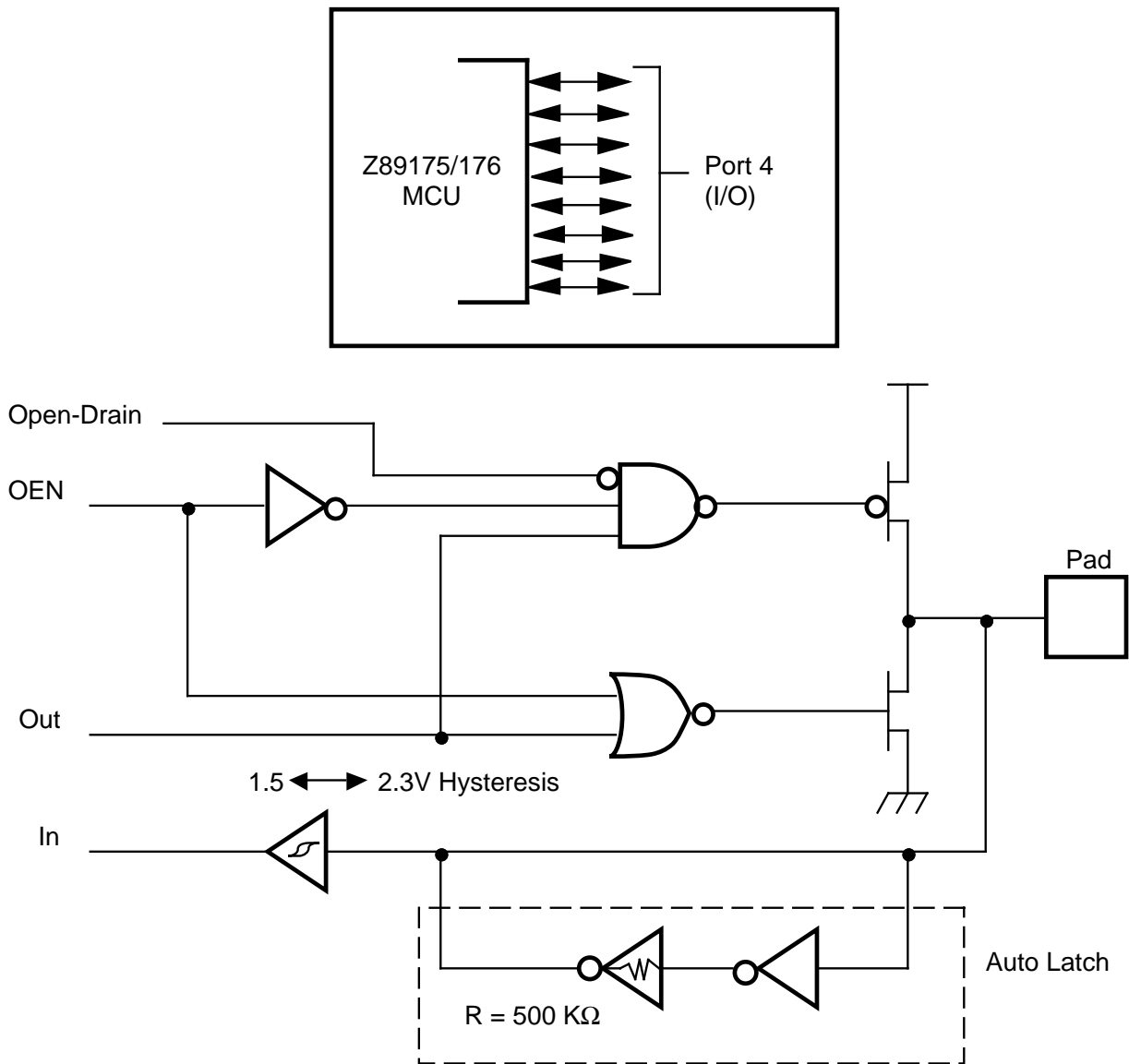
Figure 15. Port 4 Configuration
