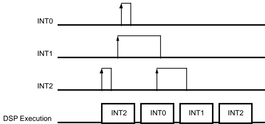
Figure 33. DSP Interrupt Priority Structure
