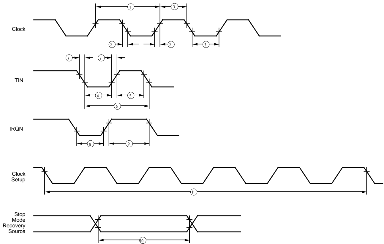
Figure 8. Additional Timing
