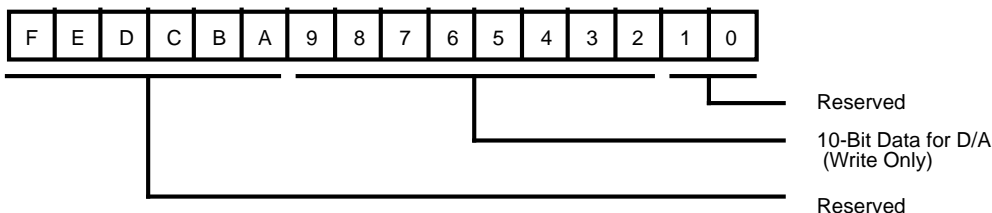
Figure 35. EXT5 Register D/A Mode Definition
