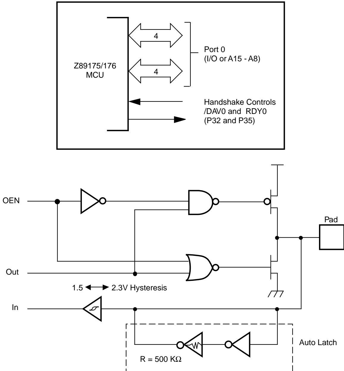
Figure 11. Port 0 Configuration
