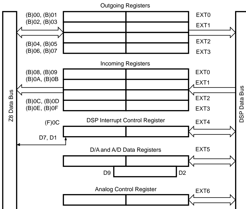
Figure 31. Z8-DSP Interface
