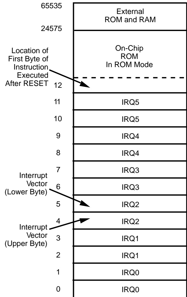
Figure 17. Program Memory
