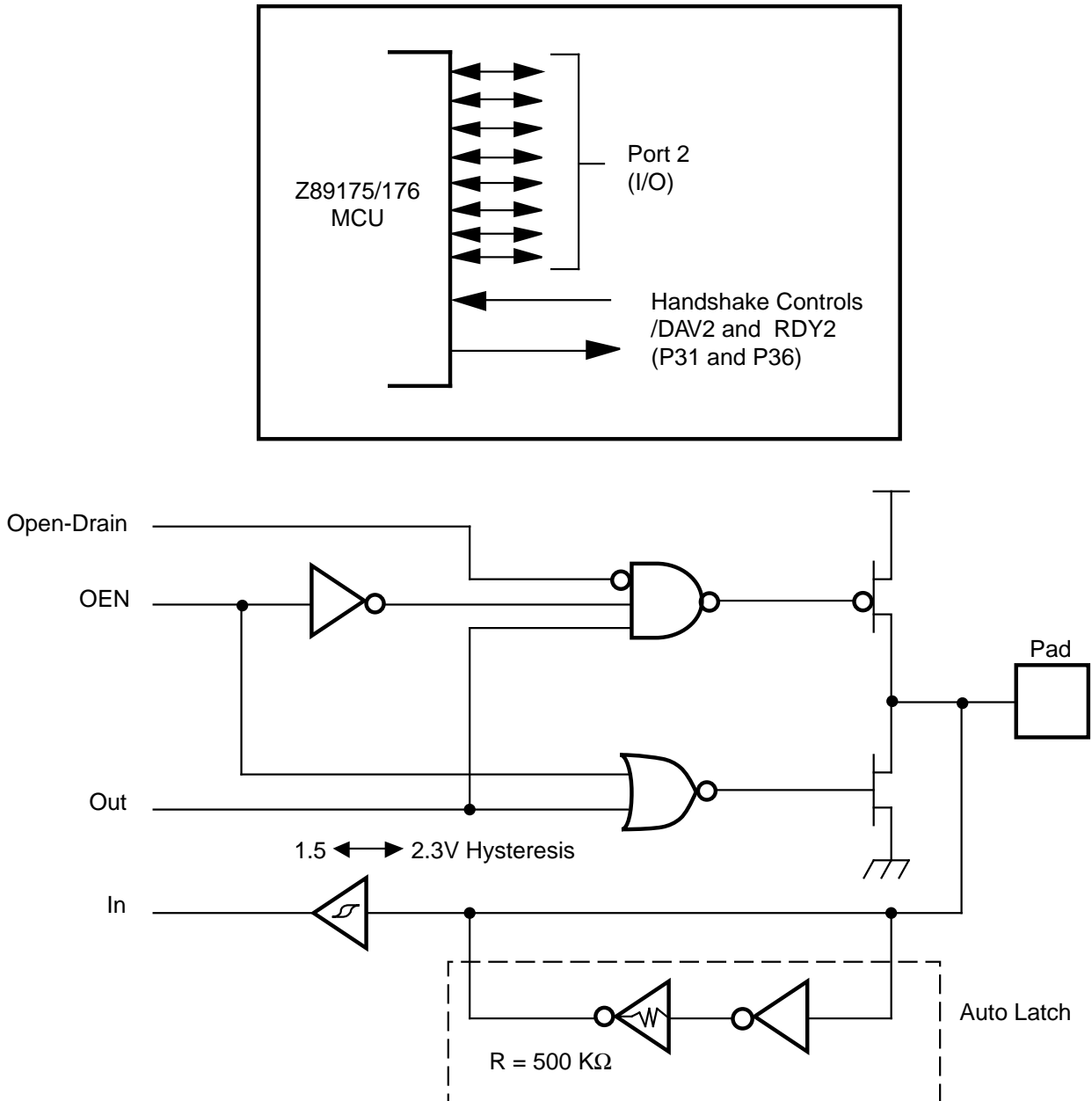
Figure 13. Port 2 Configuration
