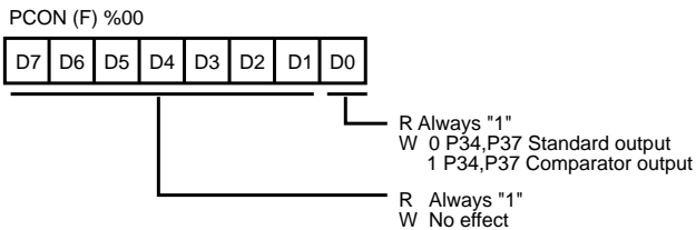
Figure 59. Port Configuration Register (PCON) (F) 00H [Write-Only]
