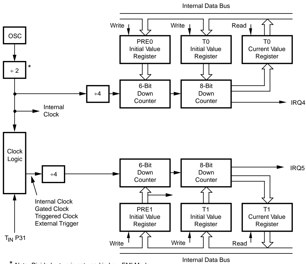
Figure 13. Counter/Timers Block Diagram
