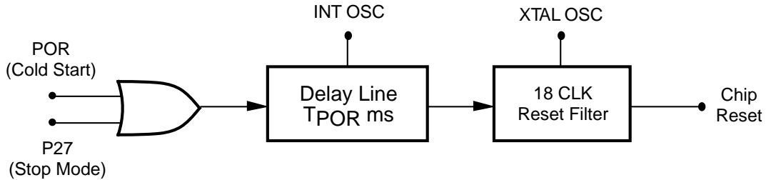
Figure 9. Internal Reset Configuration
