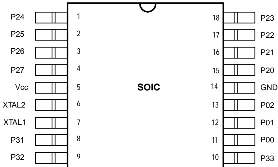
Figure 3. 18-Pin SOIC Pin Configuration
