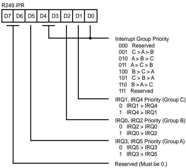
Figure 25. Interrupt Priority Register (F9 H : Write Only)
