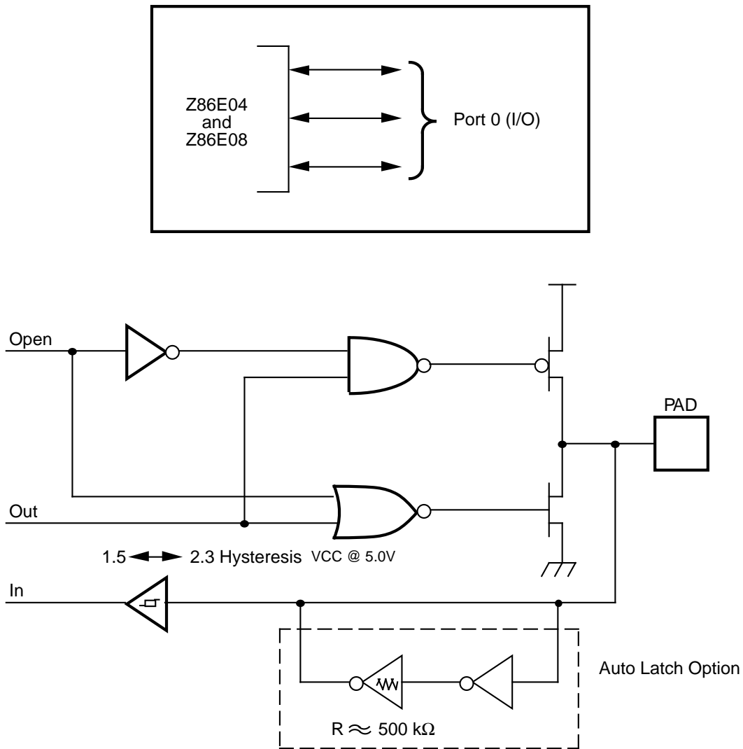
Figure 6. Port 0 Configuration
