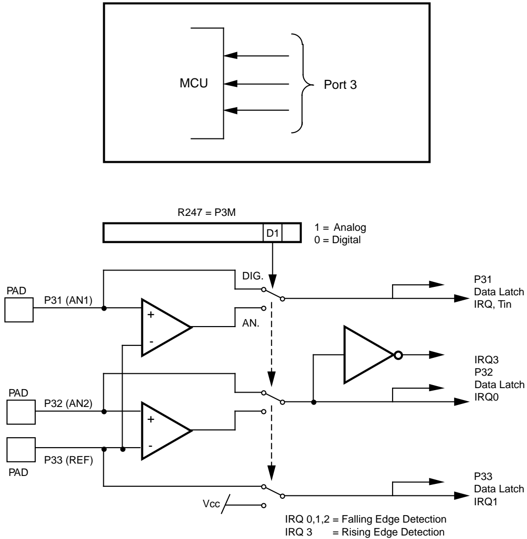
Figure 8. Port 3 Configuration
