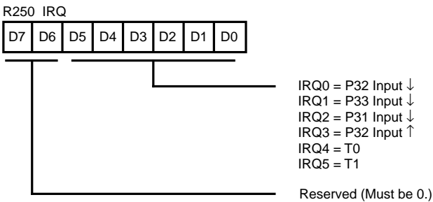
Figure 26. Interrupt Request Register (FA H : Read/Write)
