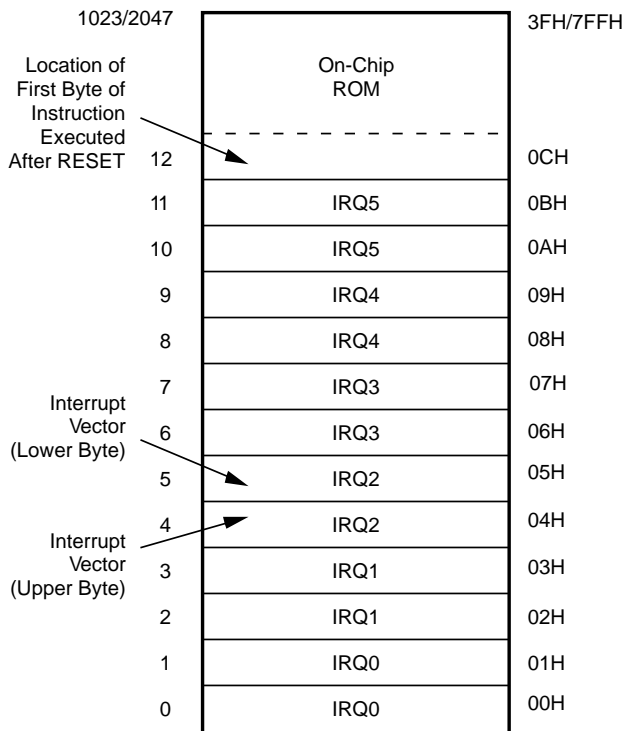
Figure 10. Program Memory Map
