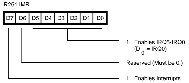
Figure 27. Interrupt Mask Register (FB H : Read/Write)
