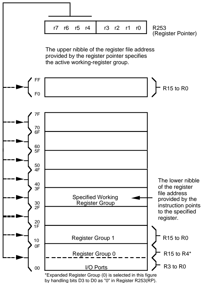
Figure 12. Register Pointer
