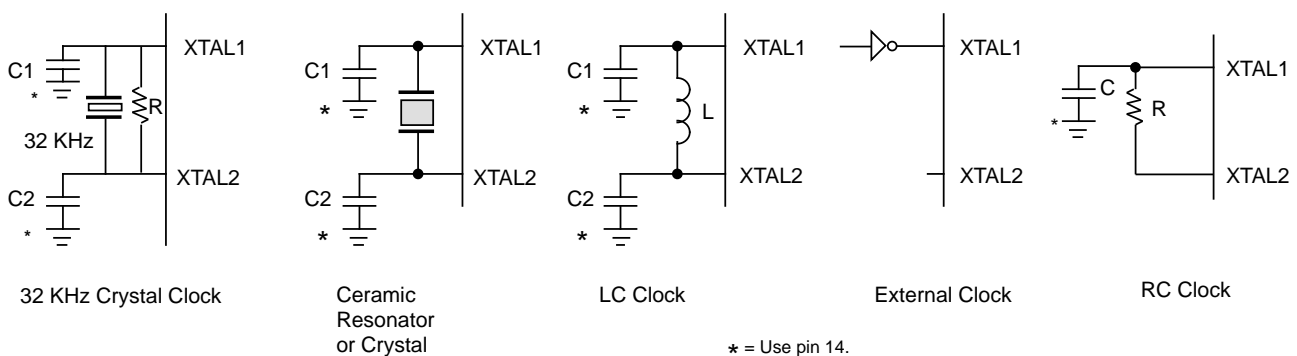
Figure 15. Oscillator Configuration
