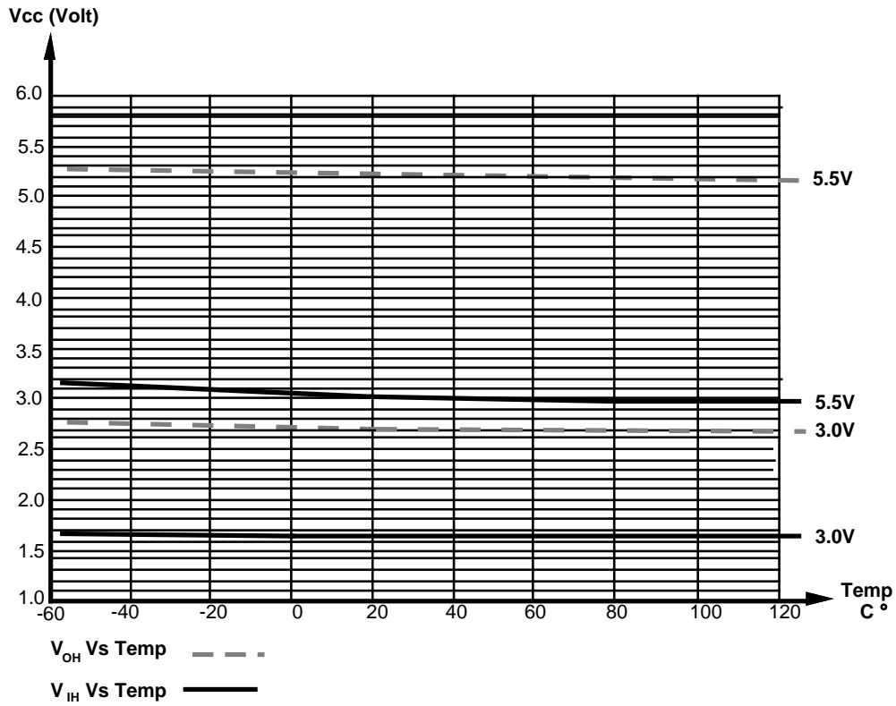
Figure 32. V IH , V OH vs. Temperature
