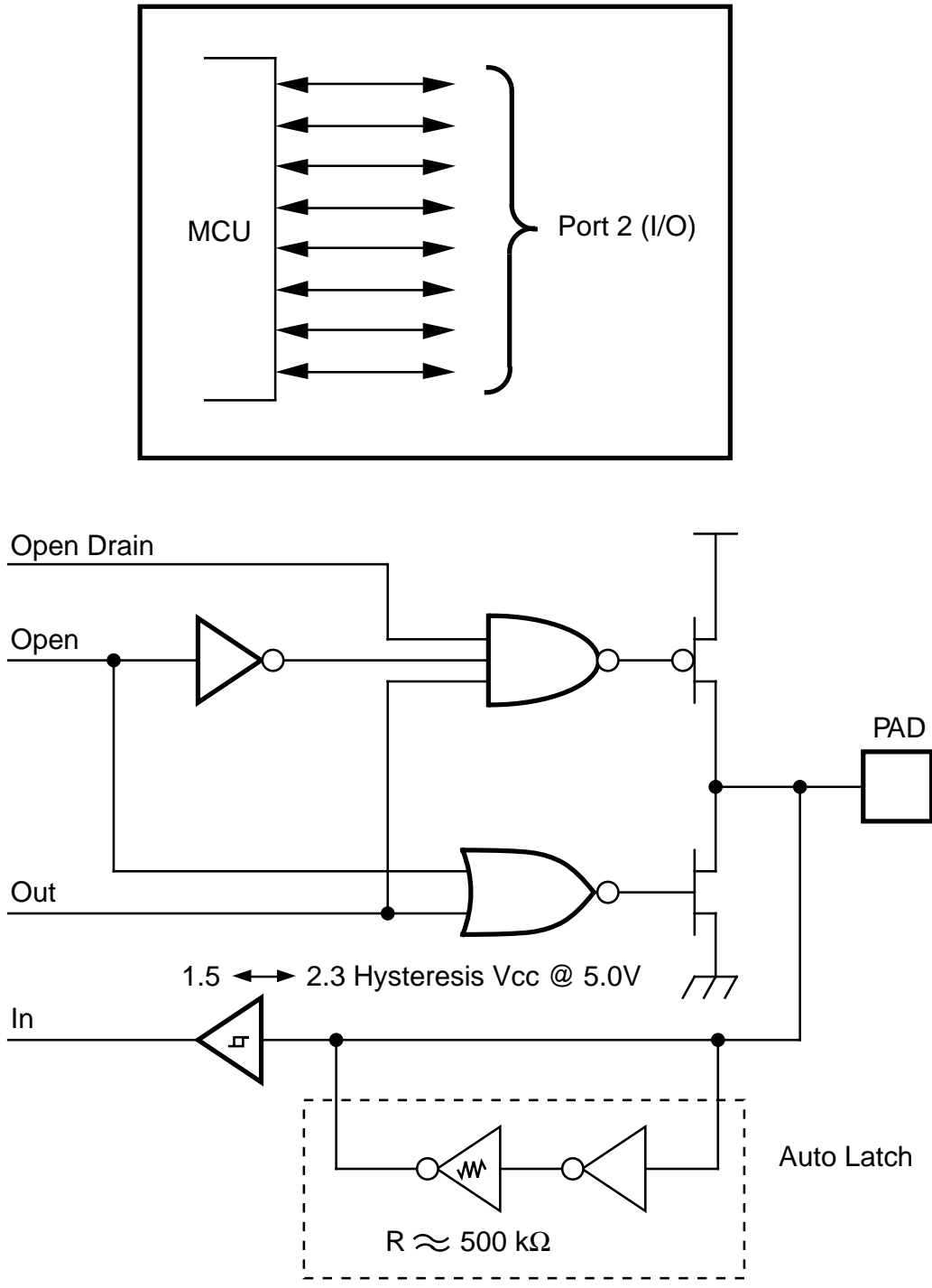
Figure 7. Port 2 Configuration
