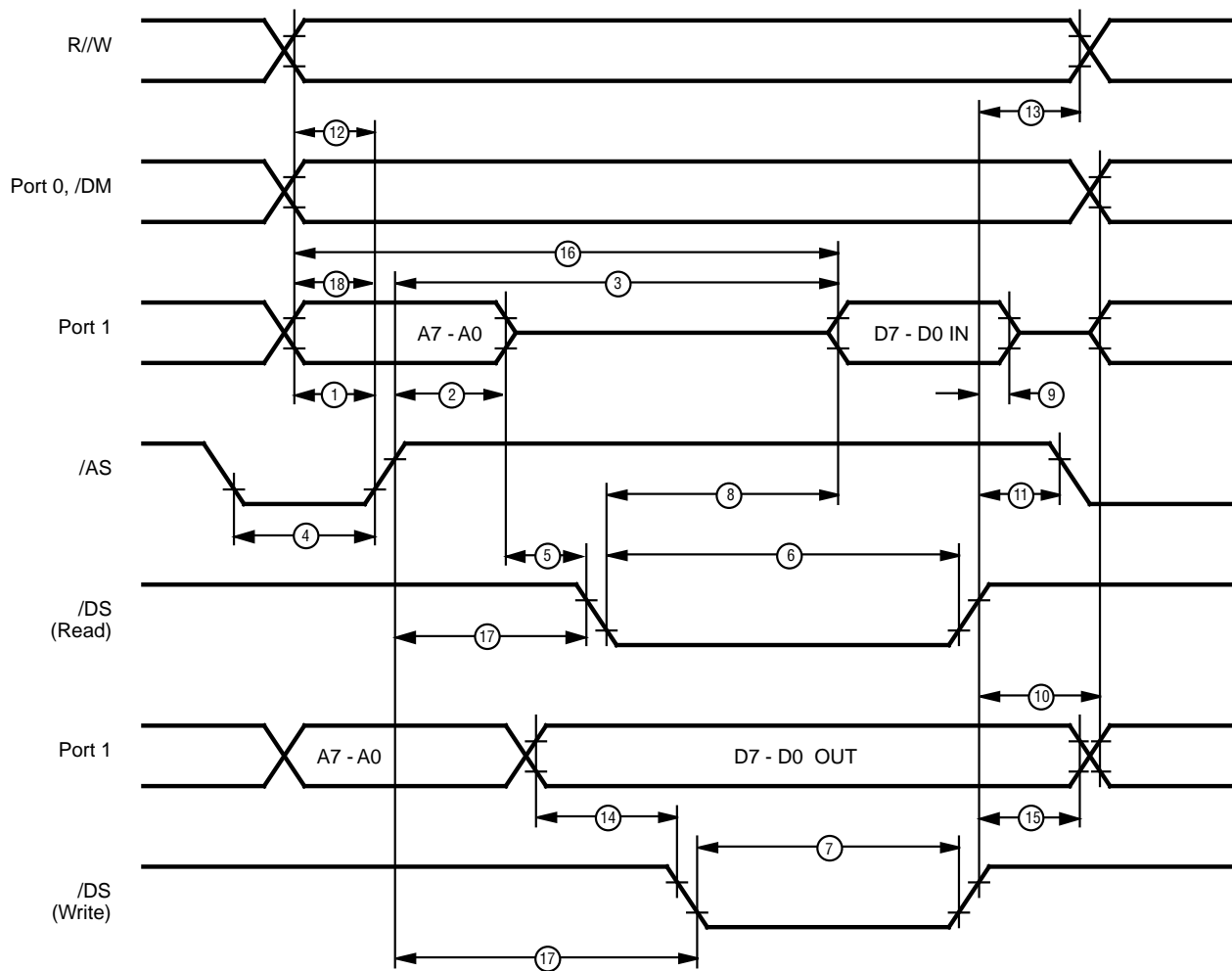
Figure 24. External I/O or Memory Read/Write Timing
