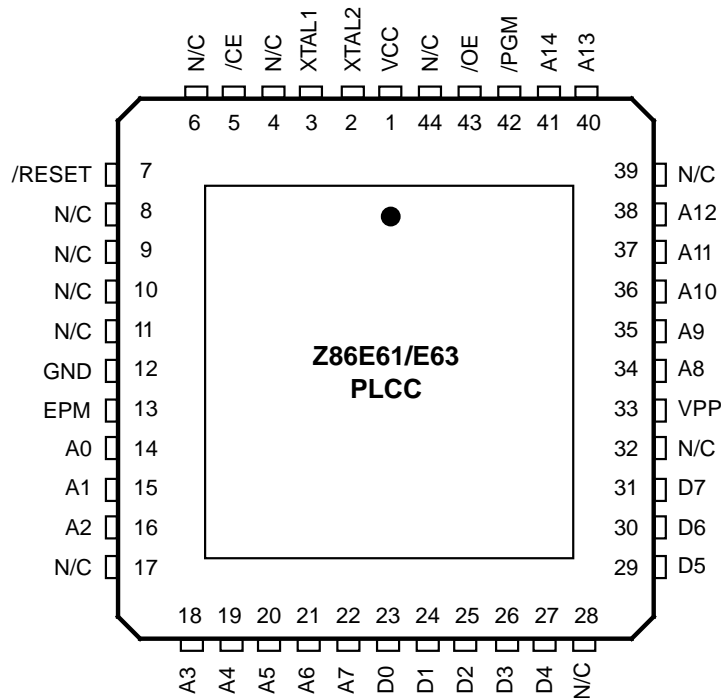
Figure 5. 44-Pin PLCC Pin Configuration
