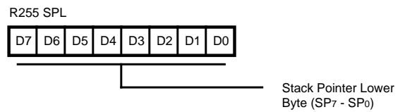
Figure 43. Stack Pointer Register (FF H : Read/Write)
