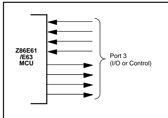
Figure 9. Port 3 Configuration
