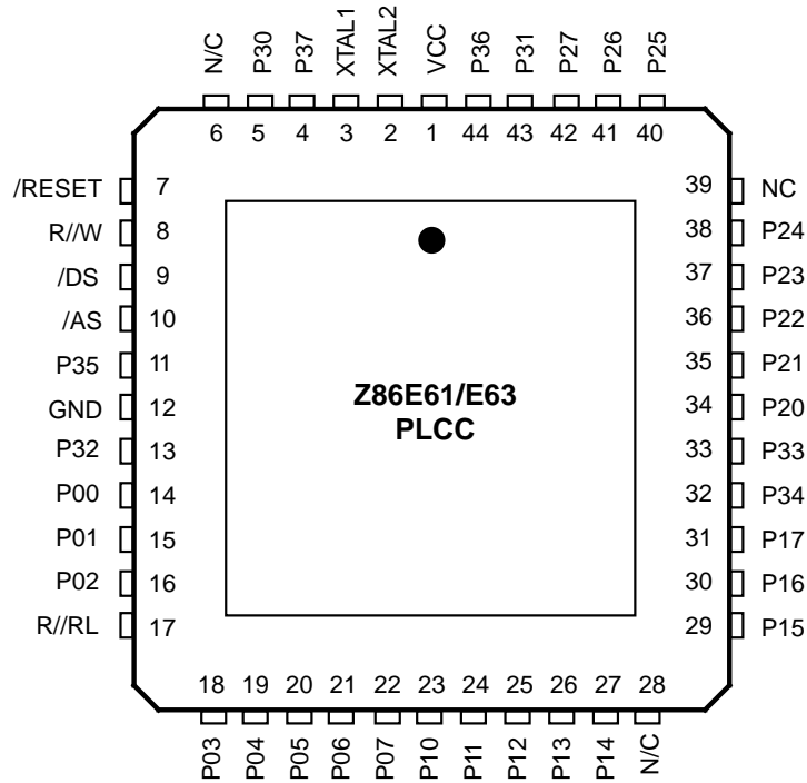
Figure 3. 44-Pin PLCC Pin Configuration
