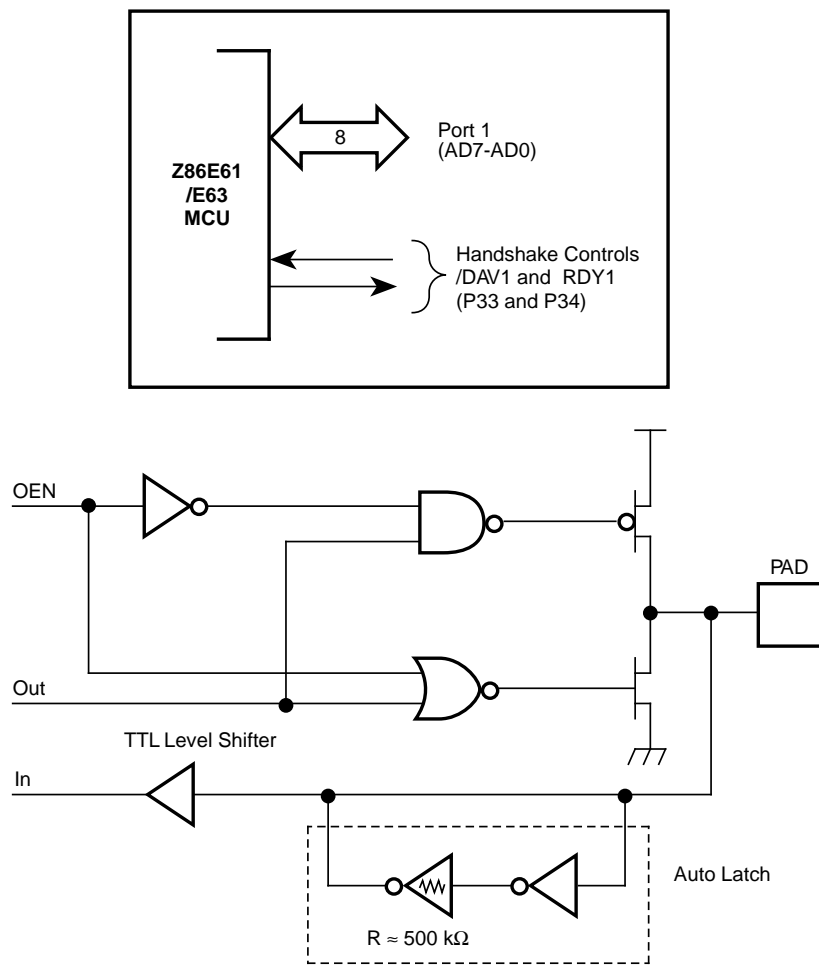
Figure 7. Port 1 Configuration
