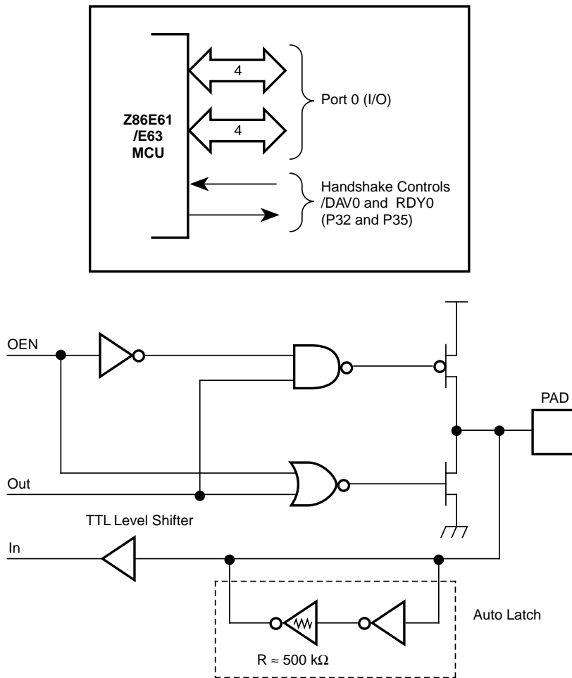
Figure 6. Port 0 Configuration
