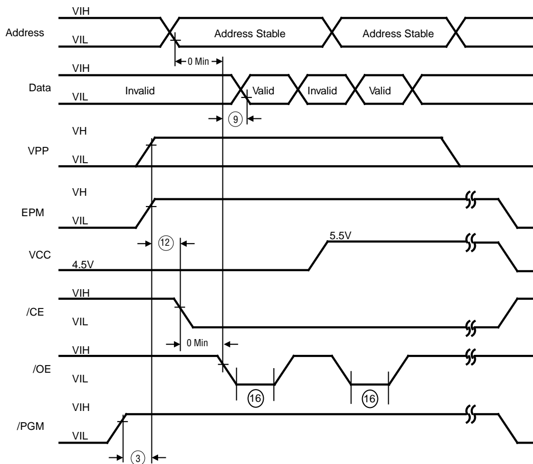
Figure 18. EPROM Read
