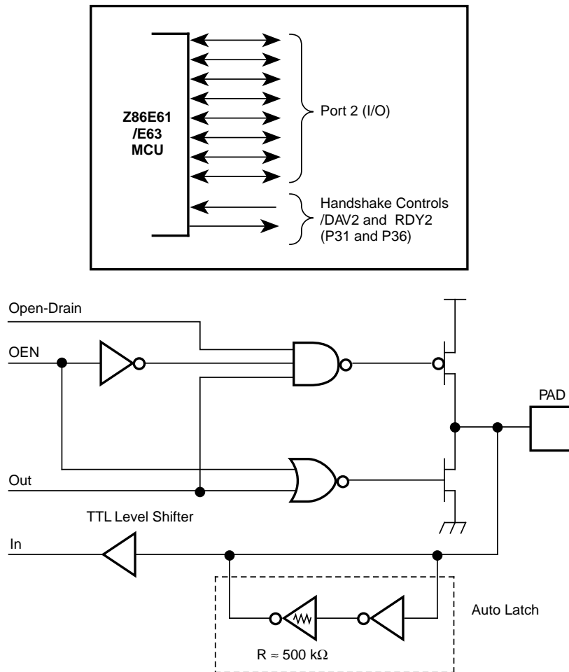
Figure 8. Port 2 Configuration
