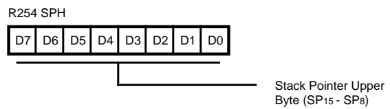
Figure 42. Stack Pointer Register (FE H : Read/Write)
