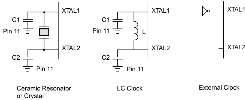
Figure 17. Oscillator Configuration
