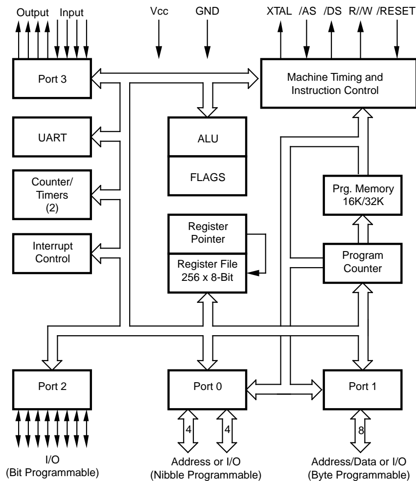
Figure 1. Z86E61/E63 Functional Block Diagram
