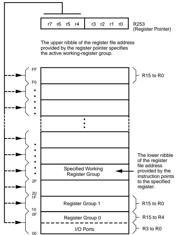
Figure 14. Register Pointer
