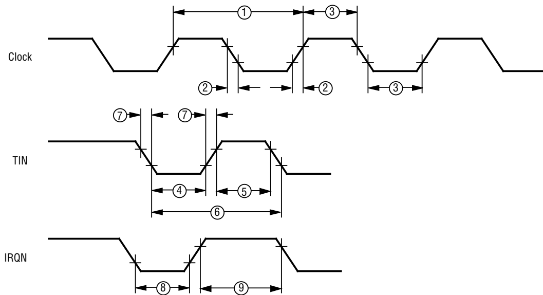
Figure 25. Additional Timing
