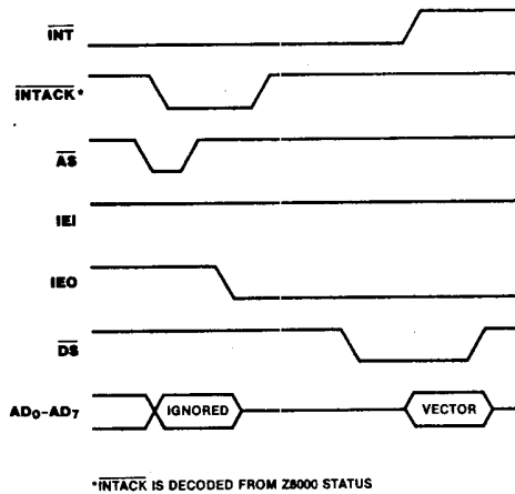
Figure 7-5. Z8036 (Z-C10) Interrupt Acknowledge Timing
