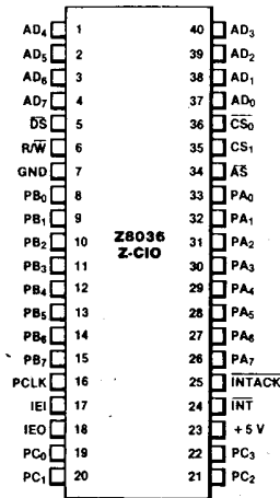
Figure 7-2. Z8036 (Z-CIO) Pin Assignments
