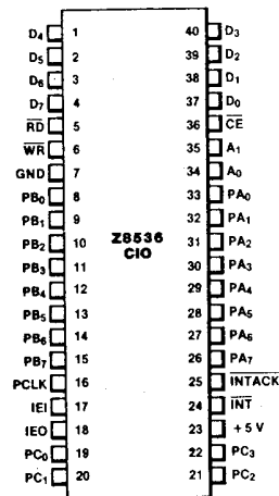
Figure 8-2. Z8536 (CIO) Pin Assignments
