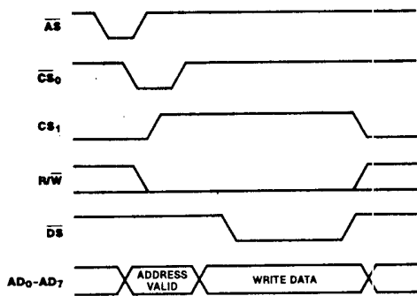
Figure 7-4. Z8036 (Z-C10) Write Cycle Timing
