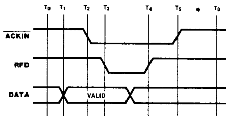
Figure 3-4. Strobed Input Handshake Timing Diagram
