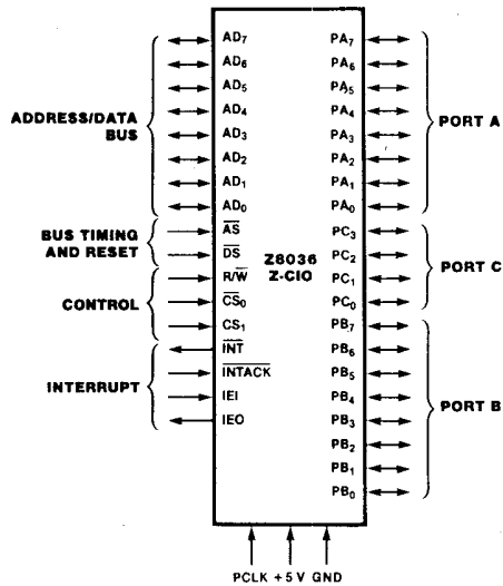
Figure 7-1. Z8036 (Z-CIO) Pin Functions
