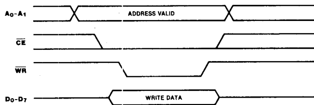
Figure 8-4. Z8536 (CIO) Write Cycle Timing
