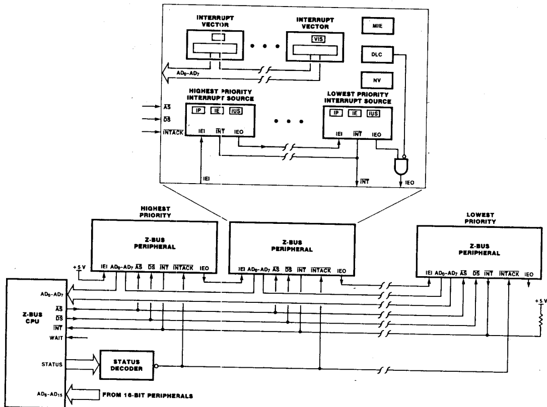
Figure 5-2. Z-BUS Interrupt Arbitration
