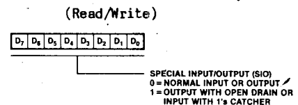
Figure 2-9. Special I/O Control Registers
