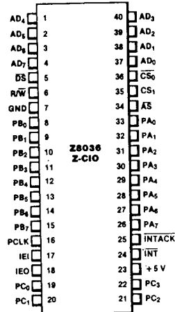
Figure 2. Pin Assignments
