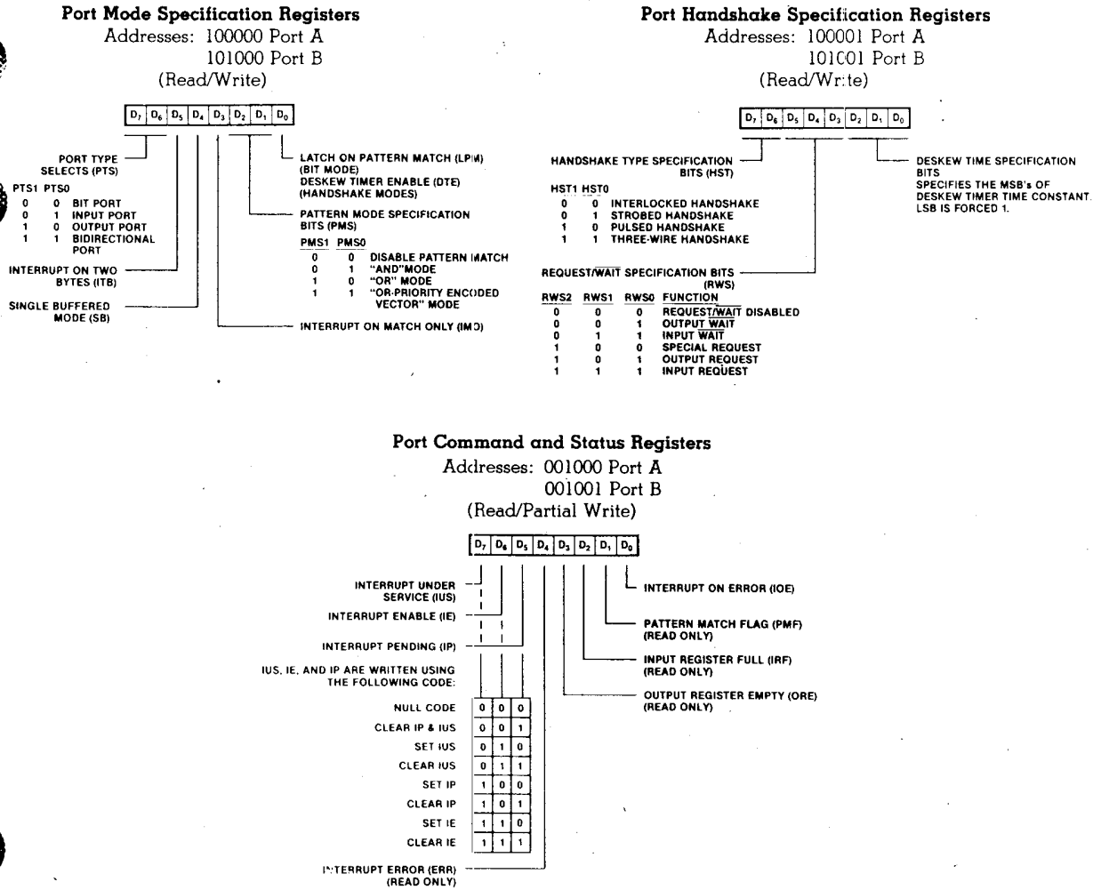
Figure B-2. Port Specification Registers
