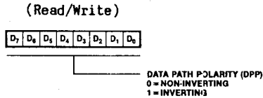
Figure 2-7. Data Path Polarity Registers
