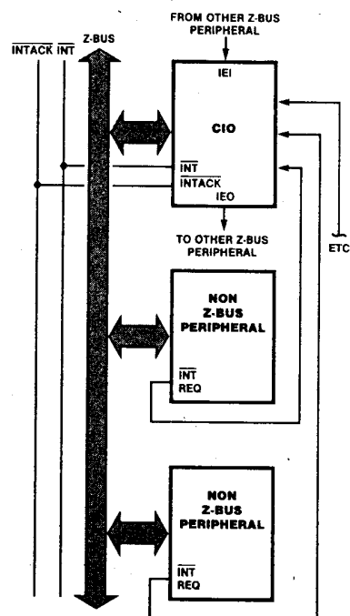
Figure 5-1. The CIO as an Interrupt Controller
