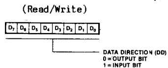
Figure 2-8. Data Direction Registers
