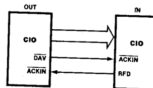
Figure 3-2. Two Interconnected CIOs Using Interlocked Handshake
