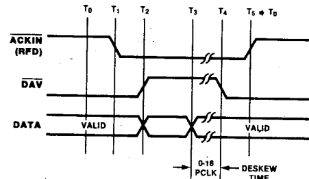
Figure 3-10. Strobed Output Handshake Timing Diagram
