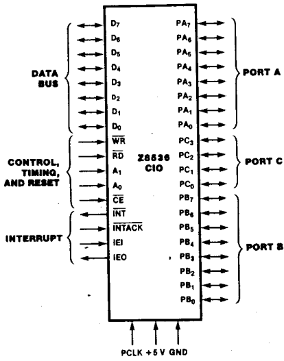
Figure 1. Pin Functions
