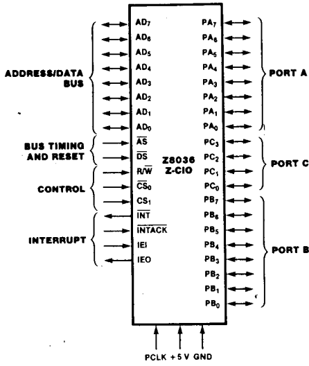
Figure 1. Pin Functions
