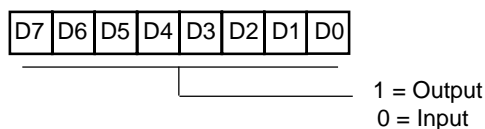
Register 0D2H PTADIR Register
