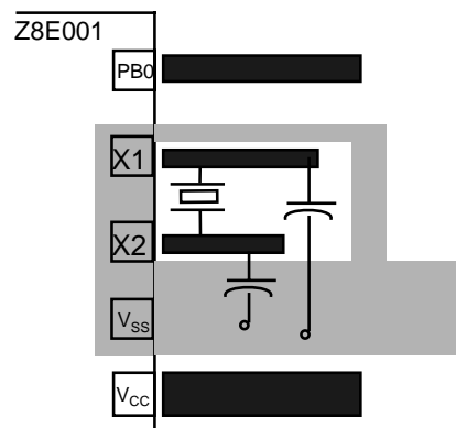
Board Design Example (Top View)
