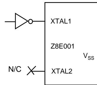
Figure 19. External Clock
