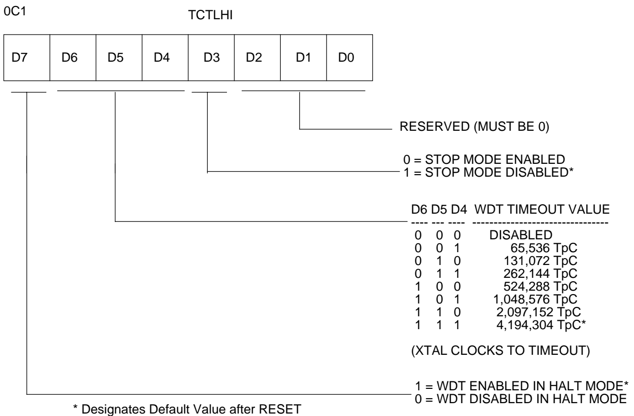
Figure 12. Z8E001 TCTLHI Register for Control of WDT
