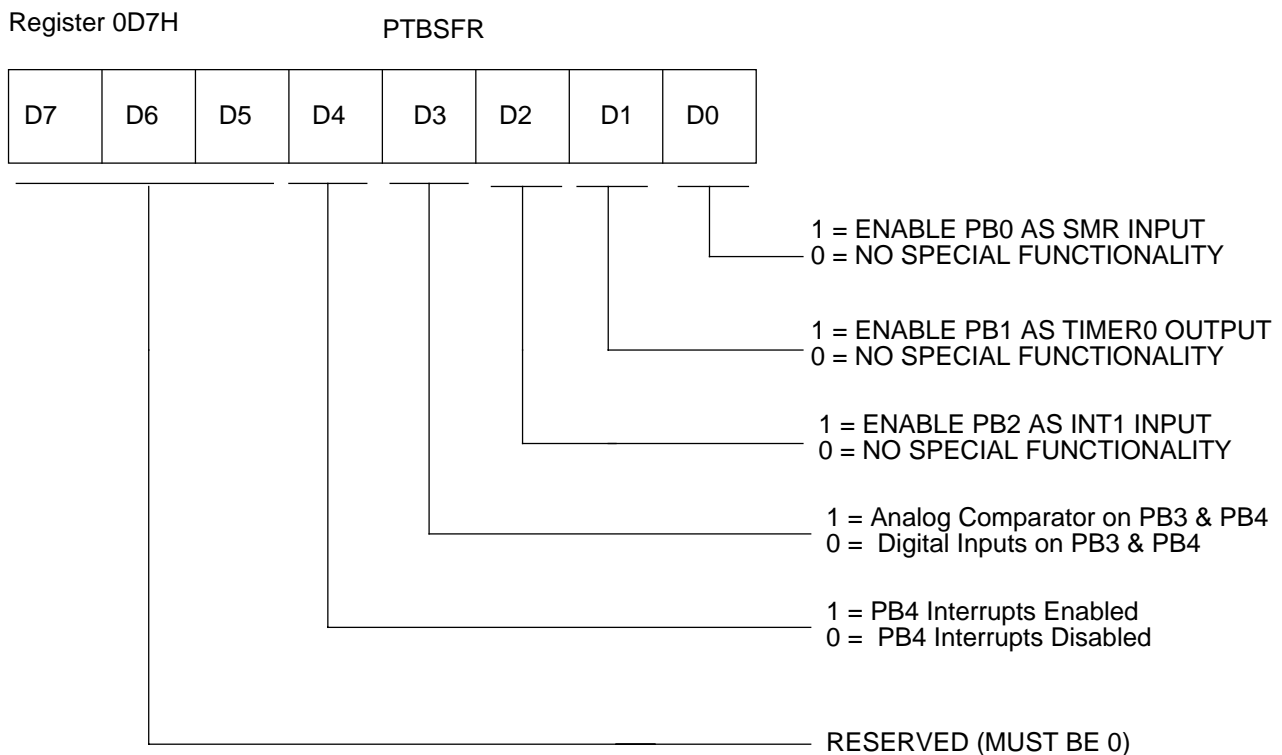
Figure 32. Port B Special Function Register
