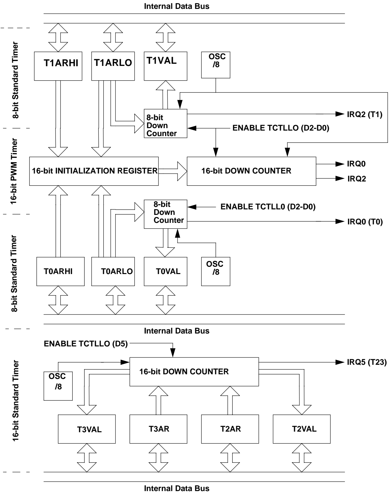
Figure 20. Timers Block Diagram
