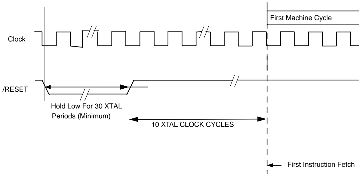
Figure 9. Reset Timing
