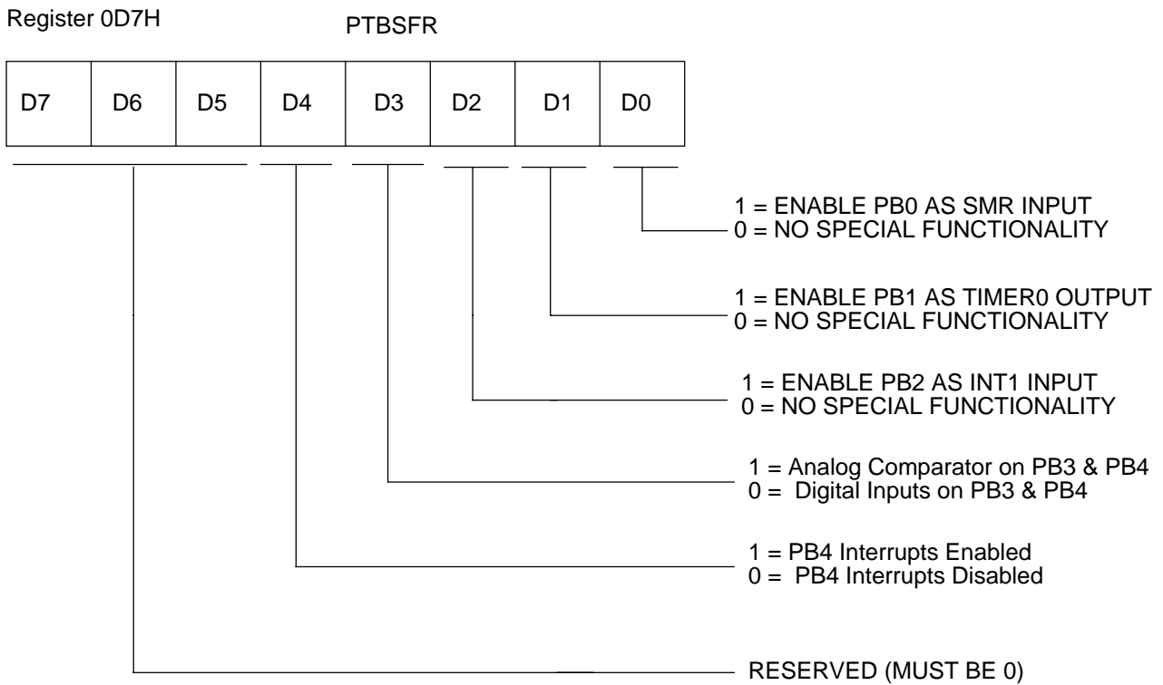
Figure 40. Port B Special Function Register
